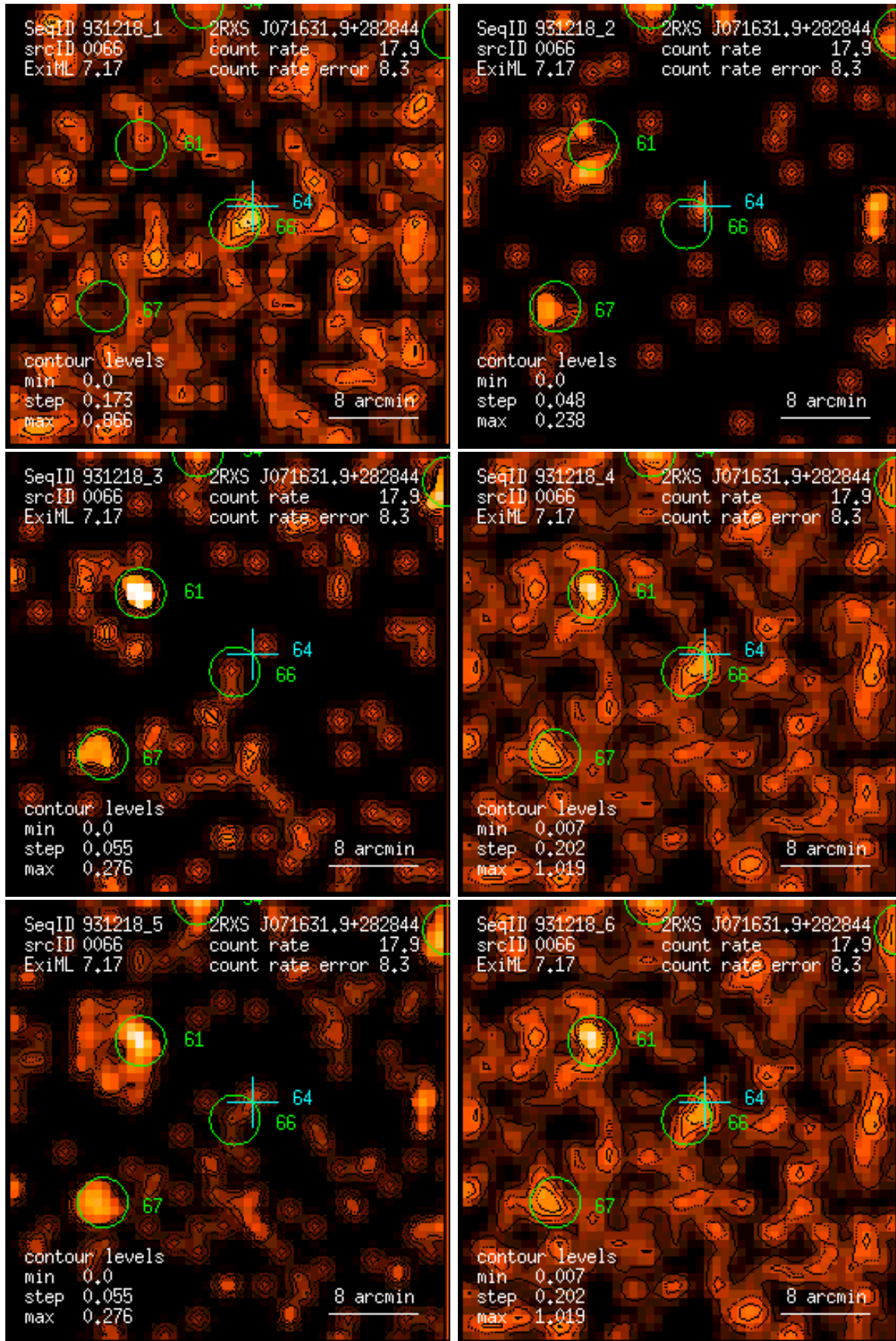
Figure 66: RASS 931218: detection 0066: band rate images, Gaussian filter: (1) PSPC channels 11 – 41, (2) 52 – 90, (3) 91 – 201, (4) 11 – 235, (5) 52 – 201, (6) 11 – 201. Broad band rates in counts/ks. Band rate contour levels in counts/ks/arcmin 2 .
