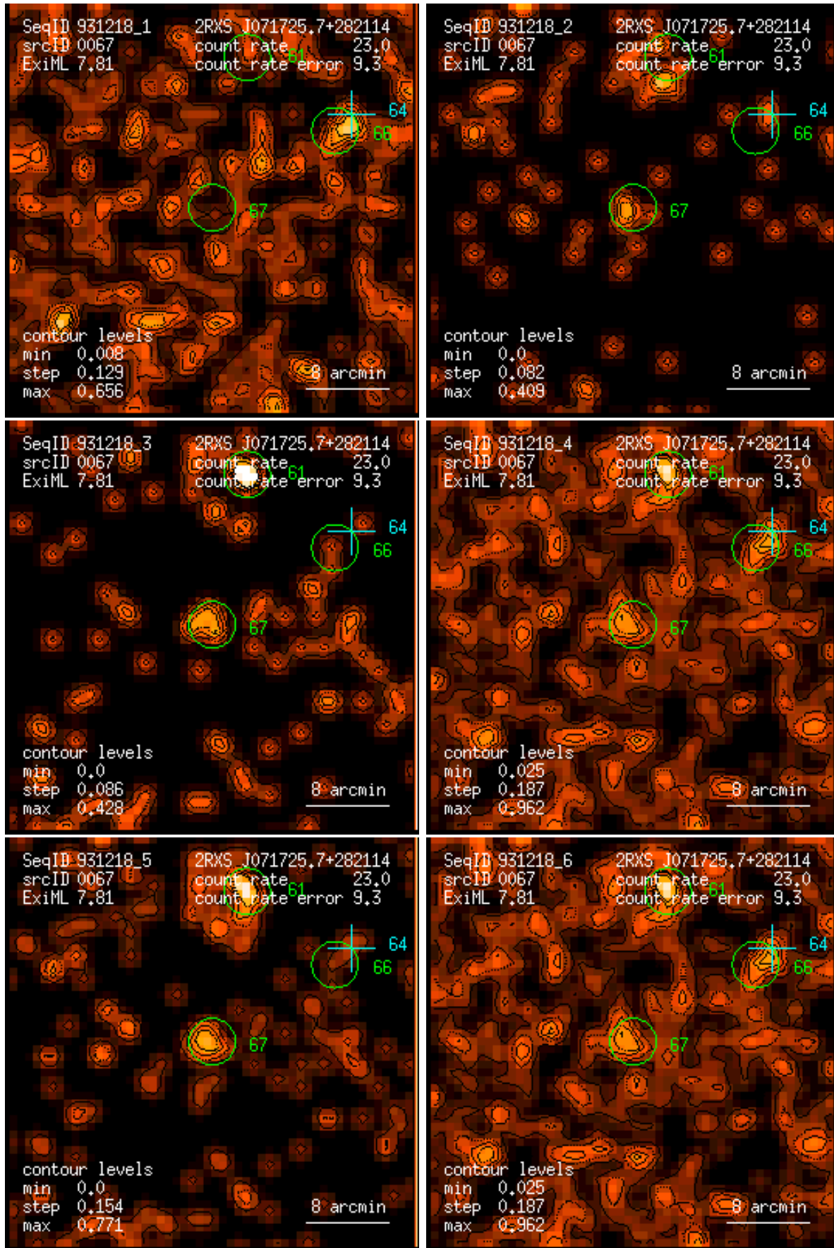
Figure 67: RASS 931218: detection 0067: band rate images, Gaussian filter: (1) PSPC channels 11 – 41, (2) 52 – 90, (3) 91 – 201, (4) 11 – 235, (5) 52 – 201, (6) 11 – 201. Broad band rates in counts/ks. Band rate contour levels in counts/ks/arcmin 2 .
