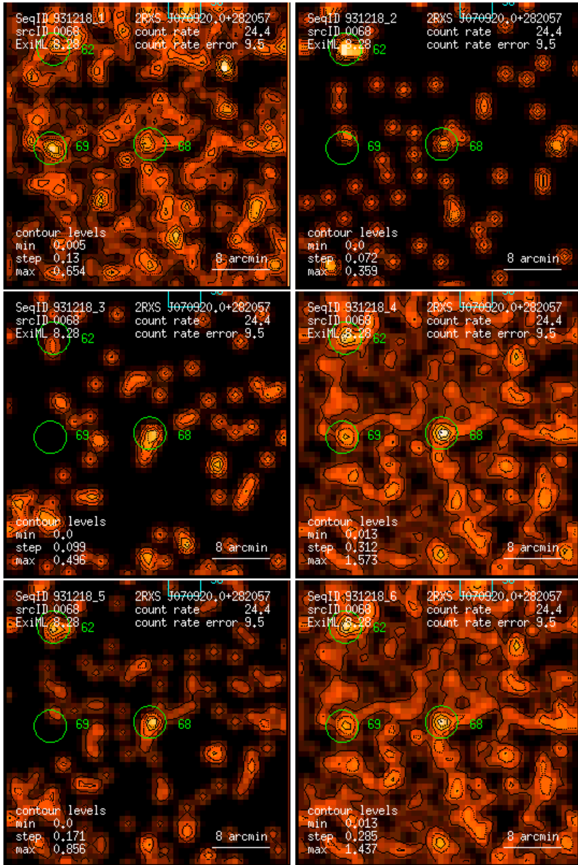
Figure 68: RASS 931218: detection 0068: band rate images, Gaussian filter: (1) PSPC channels 11 – 41, (2) 52 – 90, (3) 91 – 201, (4) 11 – 235, (5) 52 – 201, (6) 11 – 201. Broad band rates in counts/ks. Band rate contour levels in counts/ks/arcmin 2 .
