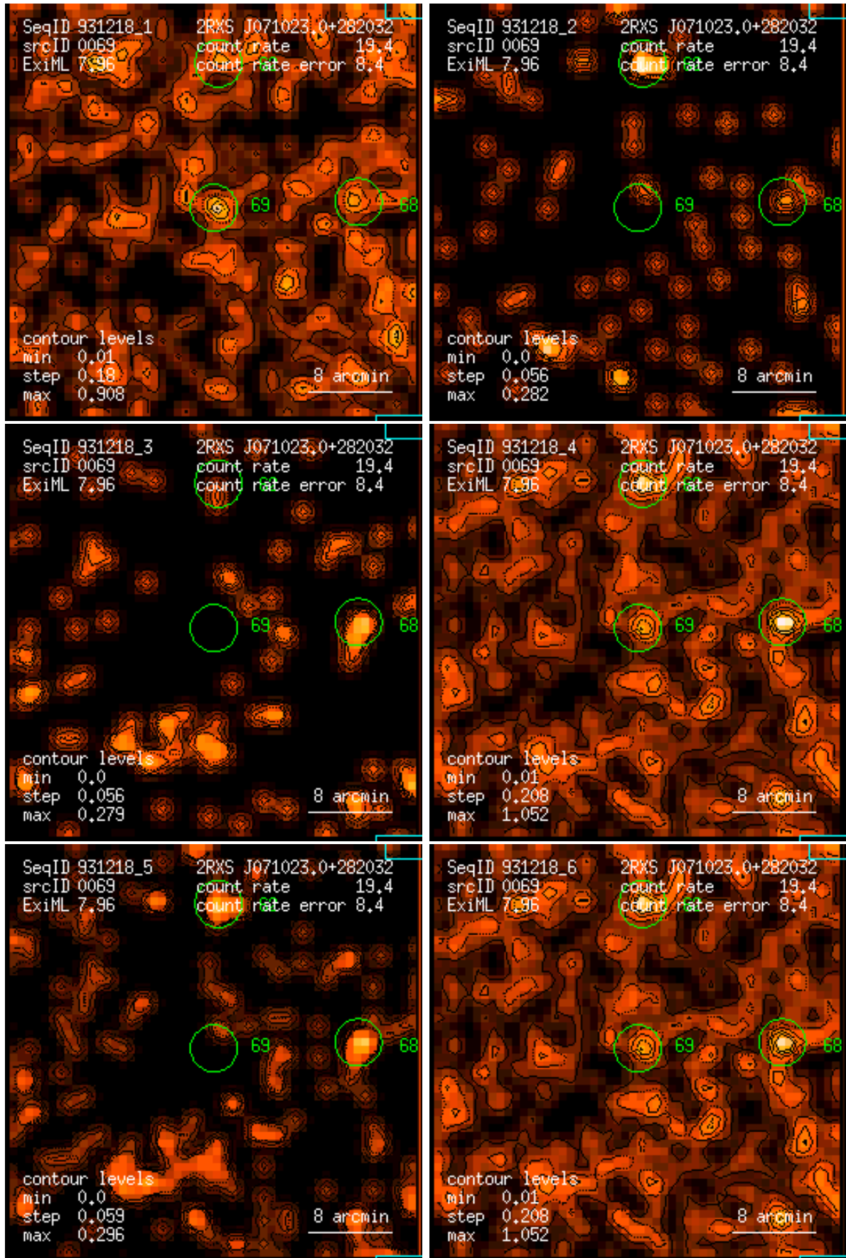
Figure 69: RASS 931218: detection 0069: band rate images, Gaussian filter: (1) PSPC channels 11 – 41, (2) 52 – 90, (3) 91 – 201, (4) 11 – 235, (5) 52 – 201, (6) 11 – 201. Broad band rates in counts/ks. Band rate contour levels in counts/ks/arcmin 2 .
