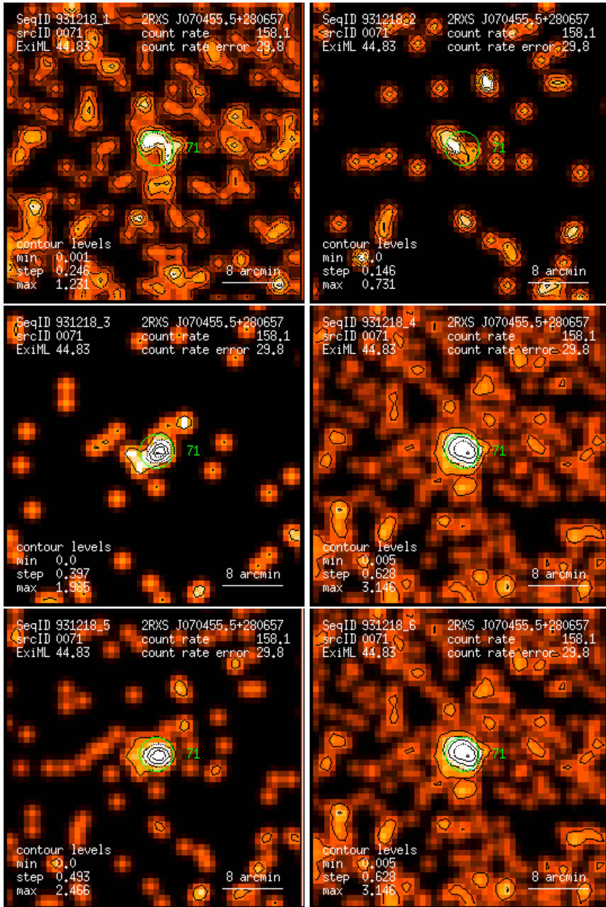
Figure 71: RASS 931218: detection 0071: band rate images, Gaussian filter: (1) PSPC channels 11 – 41, (2) 52 – 90, (3) 91 – 201, (4) 11 – 235, (5) 52 – 201, (6) 11 – 201. Broad band rates in counts/ks. Band rate contour levels in counts/ks/arcmin 2 .
