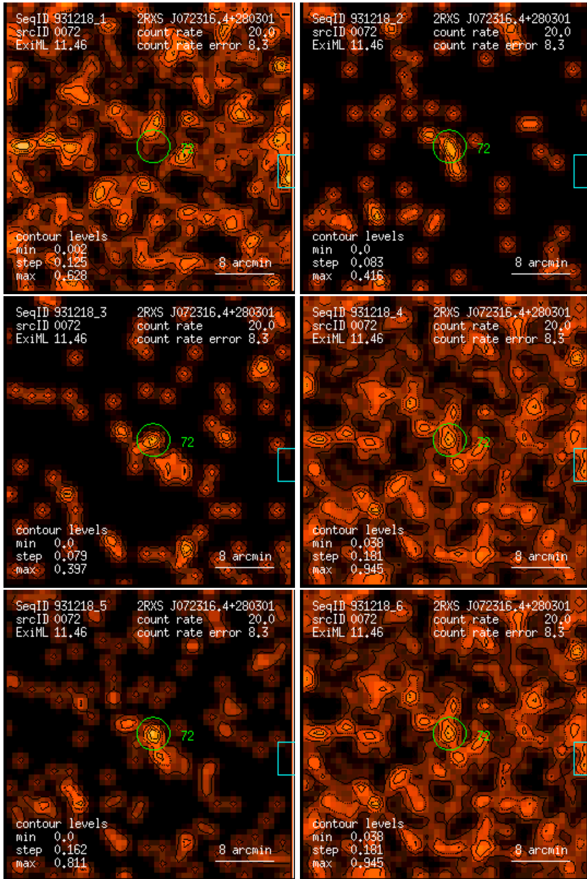
Figure 72: RASS 931218: detection 0072: band rate images, Gaussian filter: (1) PSPC channels 11 – 41, (2) 52 – 90, (3) 91 – 201, (4) 11 – 235, (5) 52 – 201, (6) 11 – 201. Broad band rates in counts/ks. Band rate contour levels in counts/ks/arcmin 2 .
