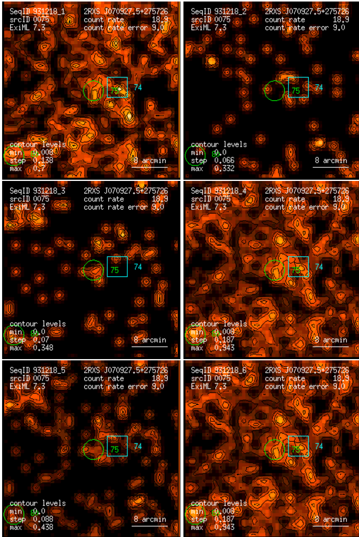
Figure 75: RASS 931218: detection 0075: band rate images, Gaussian filter: (1) PSPC channels 11 – 41, (2) 52 – 90, (3) 91 – 201, (4) 11 – 235, (5) 52 – 201, (6) 11 – 201. Broad band rates in counts/ks. Band rate contour levels in counts/ks/arcmin 2 .
