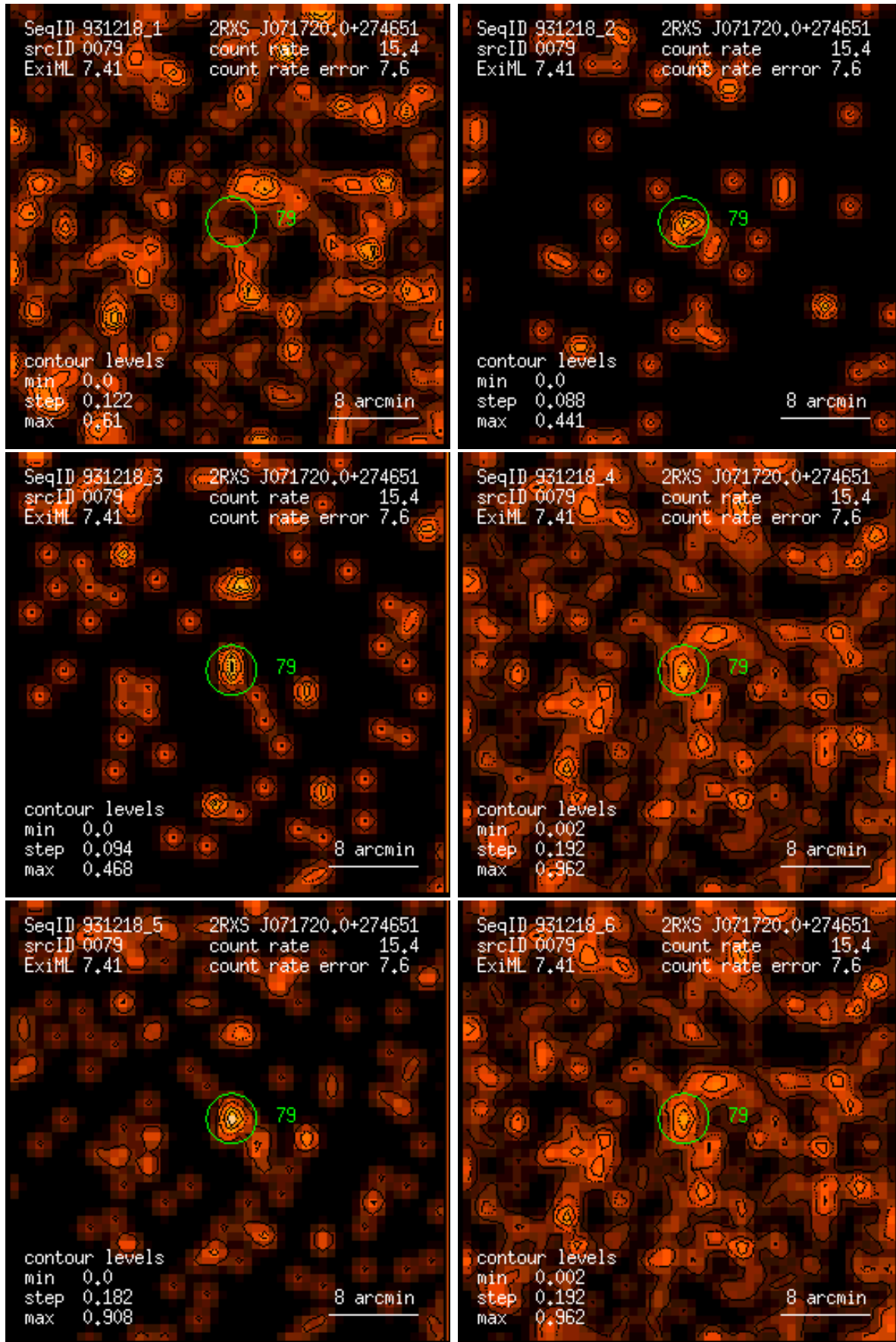
Figure 79: RASS 931218: detection 0079: band rate images, Gaussian filter: (1) PSPC channels 11 – 41, (2) 52 – 90, (3) 91 – 201, (4) 11 – 235, (5) 52 – 201, (6) 11 – 201. Broad band rates in counts/ks. Band rate contour levels in counts/ks/arcmin 2 .
