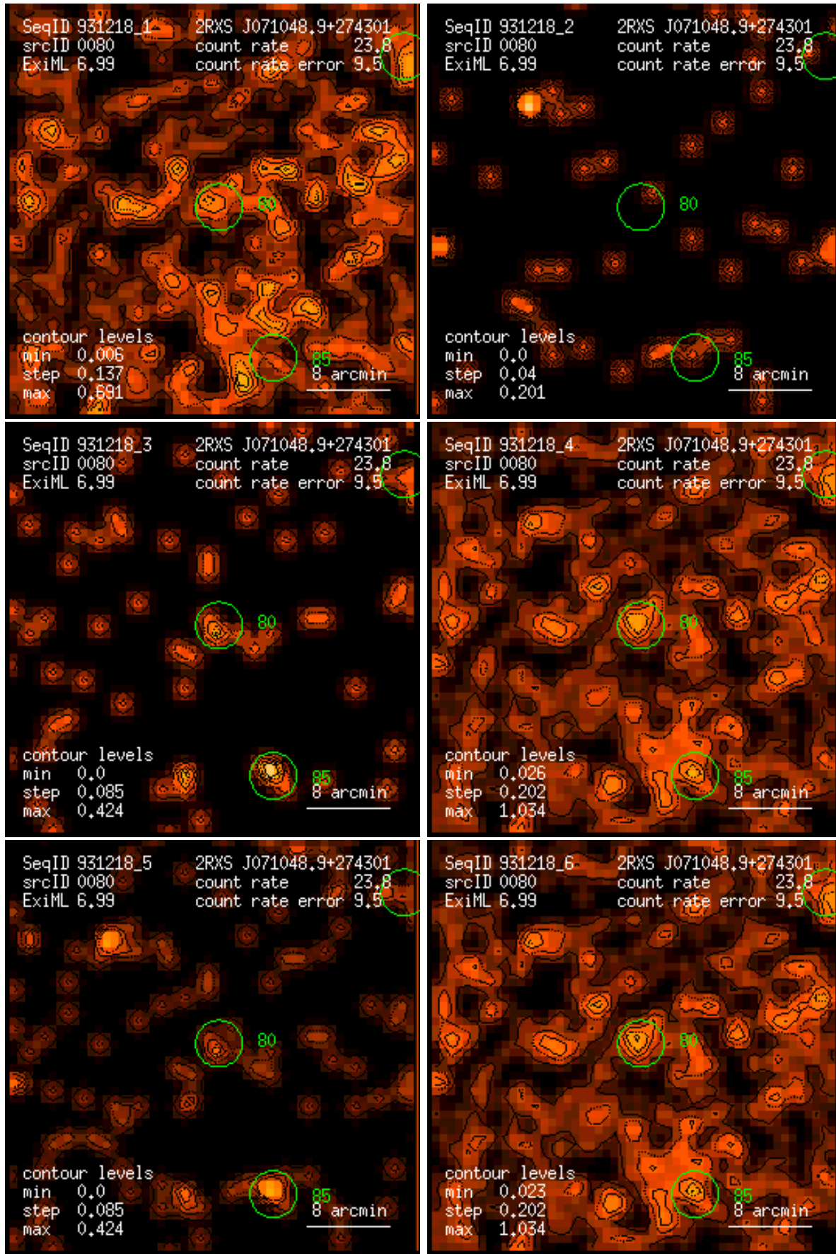
Figure 80: RASS 931218: detection 0080: band rate images, Gaussian filter: (1) PSPC channels 11 – 41, (2) 52 – 90, (3) 91 – 201, (4) 11 – 235, (5) 52 – 201, (6) 11 – 201. Broad band rates in counts/ks. Band rate contour levels in counts/ks/arcmin 2 .
