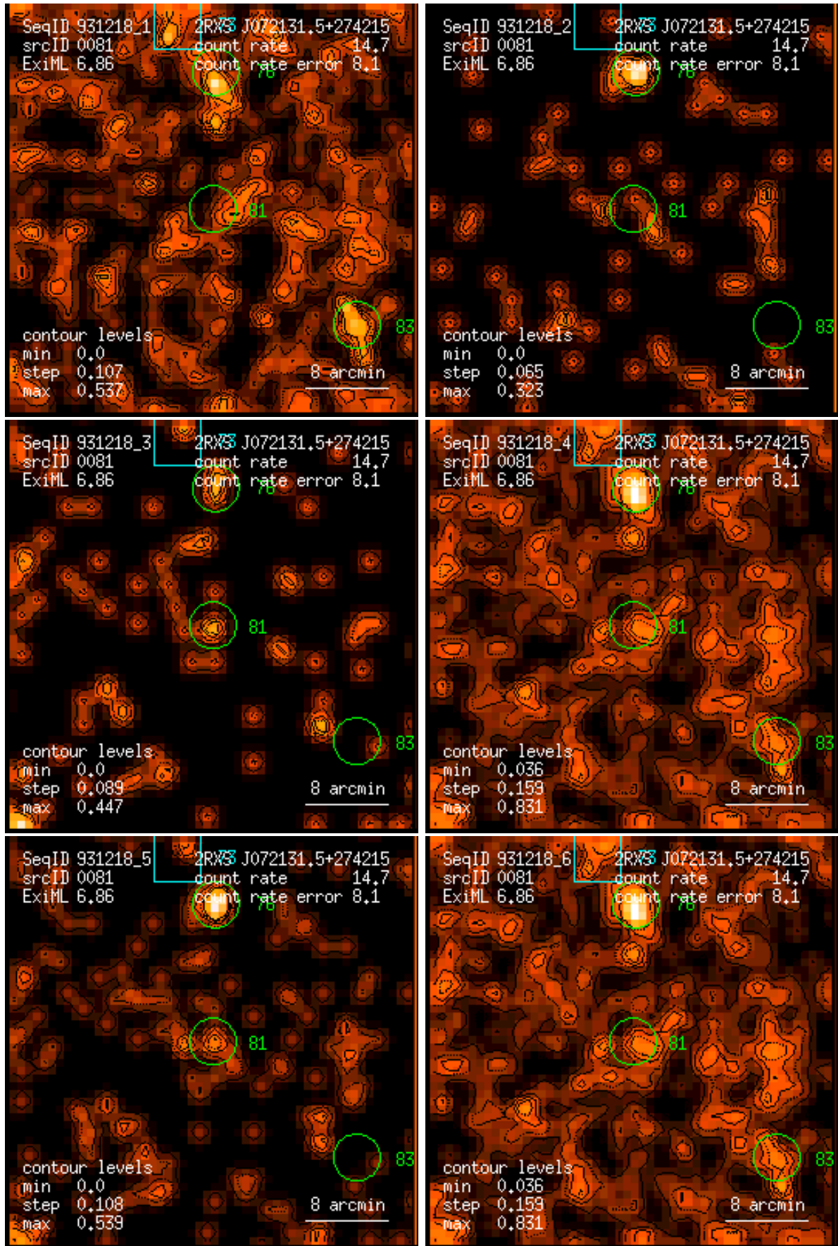
Figure 81: RASS 931218: detection 0081: band rate images, Gaussian filter: (1) PSPC channels 11 – 41, (2) 52 – 90, (3) 91 – 201, (4) 11 – 235, (5) 52 – 201, (6) 11 – 201. Broad band rates in counts/ks. Band rate contour levels in counts/ks/arcmin 2 .
