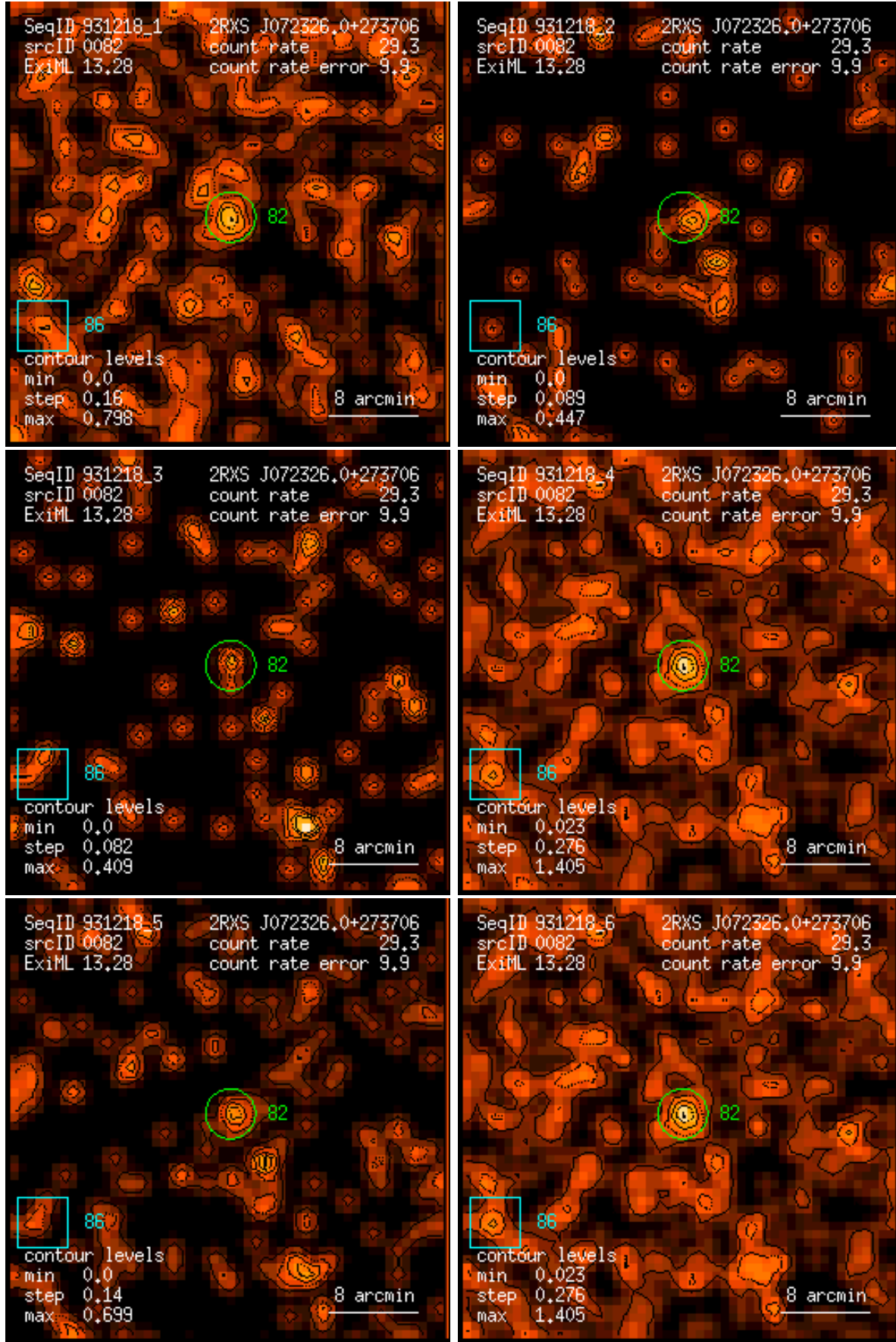
Figure 82: RASS 931218: detection 0082: band rate images, Gaussian filter: (1) PSPC channels 11 – 41, (2) 52 – 90, (3) 91 – 201, (4) 11 – 235, (5) 52 – 201, (6) 11 – 201. Broad band rates in counts/ks. Band rate contour levels in counts/ks/arcmin 2 .
