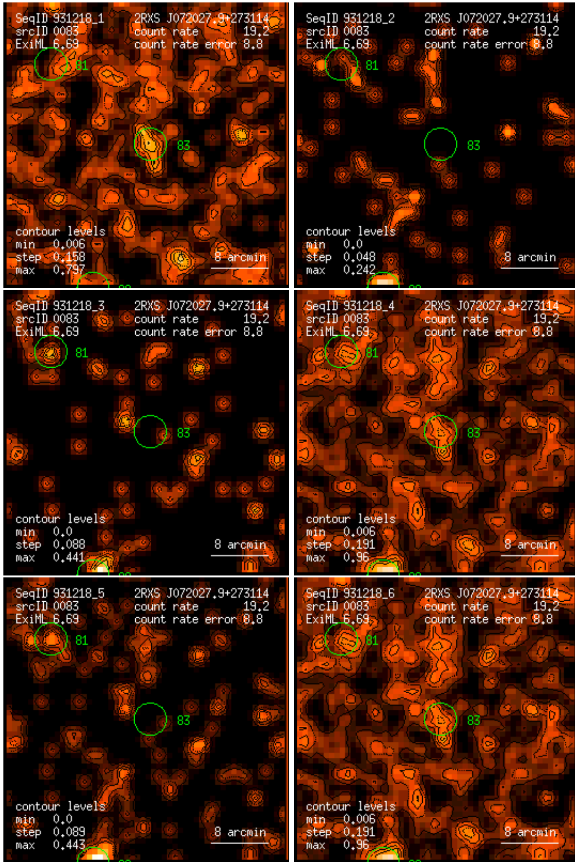
Figure 83: RASS 931218: detection 0083: band rate images, Gaussian filter: (1) PSPC channels 11 – 41, (2) 52 – 90, (3) 91 – 201, (4) 11 – 235, (5) 52 – 201, (6) 11 – 201. Broad band rates in counts/ks. Band rate contour levels in counts/ks/arcmin 2 .
