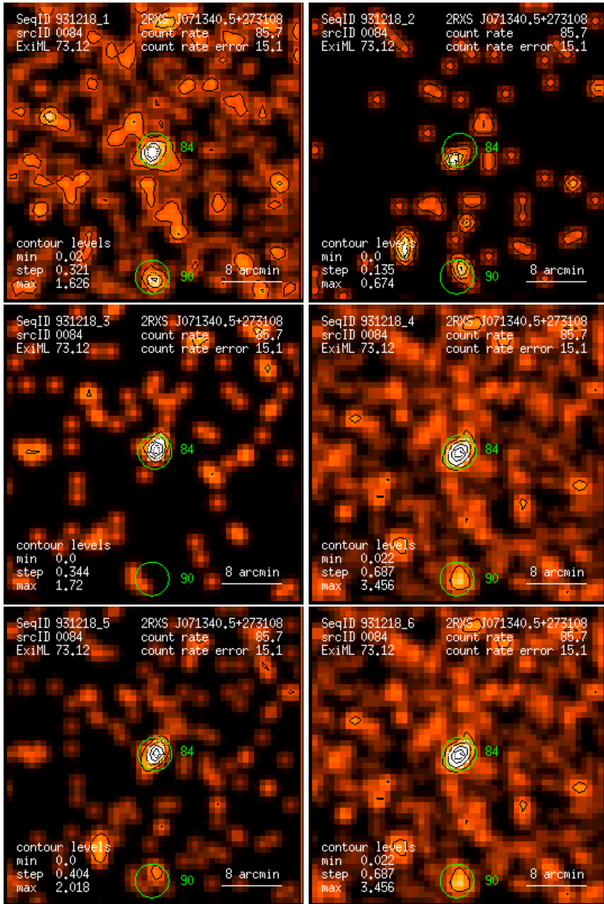
Figure 84: RASS 931218: detection 0084: band rate images, Gaussian filter: (1) PSPC channels 11 – 41, (2) 52 – 90, (3) 91 – 201, (4) 11 – 235, (5) 52 – 201, (6) 11 – 201. Broad band rates in counts/ks. Band rate contour levels in counts/ks/arcmin 2 .
