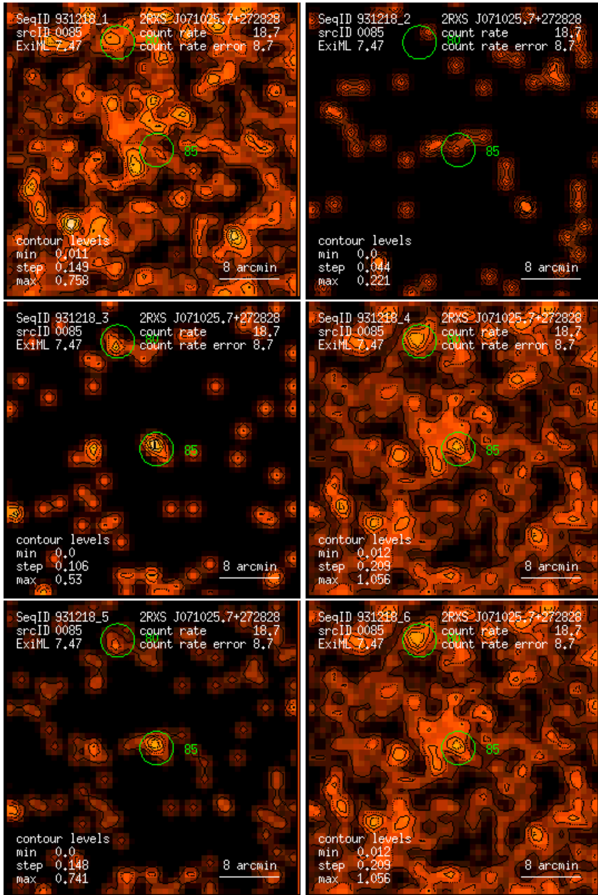
Figure 85: RASS 931218: detection 0085: band rate images, Gaussian filter: (1) PSPC channels 11 – 41, (2) 52 – 90, (3) 91 – 201, (4) 11 – 235, (5) 52 – 201, (6) 11 – 201. Broad band rates in counts/ks. Band rate contour levels in counts/ks/arcmin 2 .
