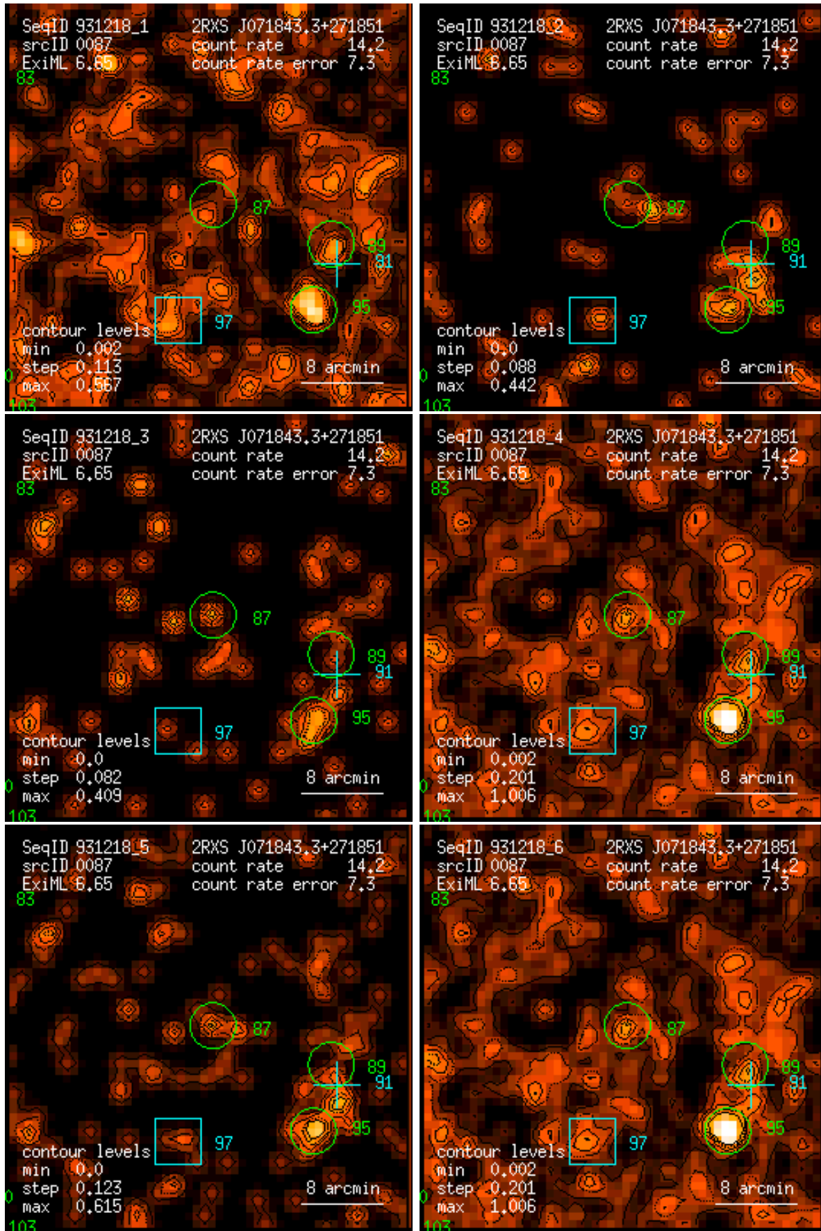
Figure 87: RASS 931218: detection 0087: band rate images, Gaussian filter: (1) PSPC channels 11 – 41, (2) 52 – 90, (3) 91 – 201, (4) 11 – 235, (5) 52 – 201, (6) 11 – 201. Broad band rates in counts/ks. Band rate contour levels in counts/ks/arcmin 2 .
