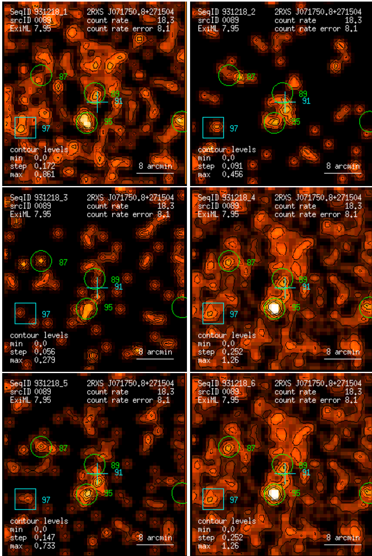
Figure 89: RASS 931218: detection 0089: band rate images, Gaussian filter: (1) PSPC channels 11 – 41, (2) 52 – 90, (3) 91 – 201, (4) 11 – 235, (5) 52 – 201, (6) 11 – 201. Broad band rates in counts/ks. Band rate contour levels in counts/ks/arcmin 2 .
