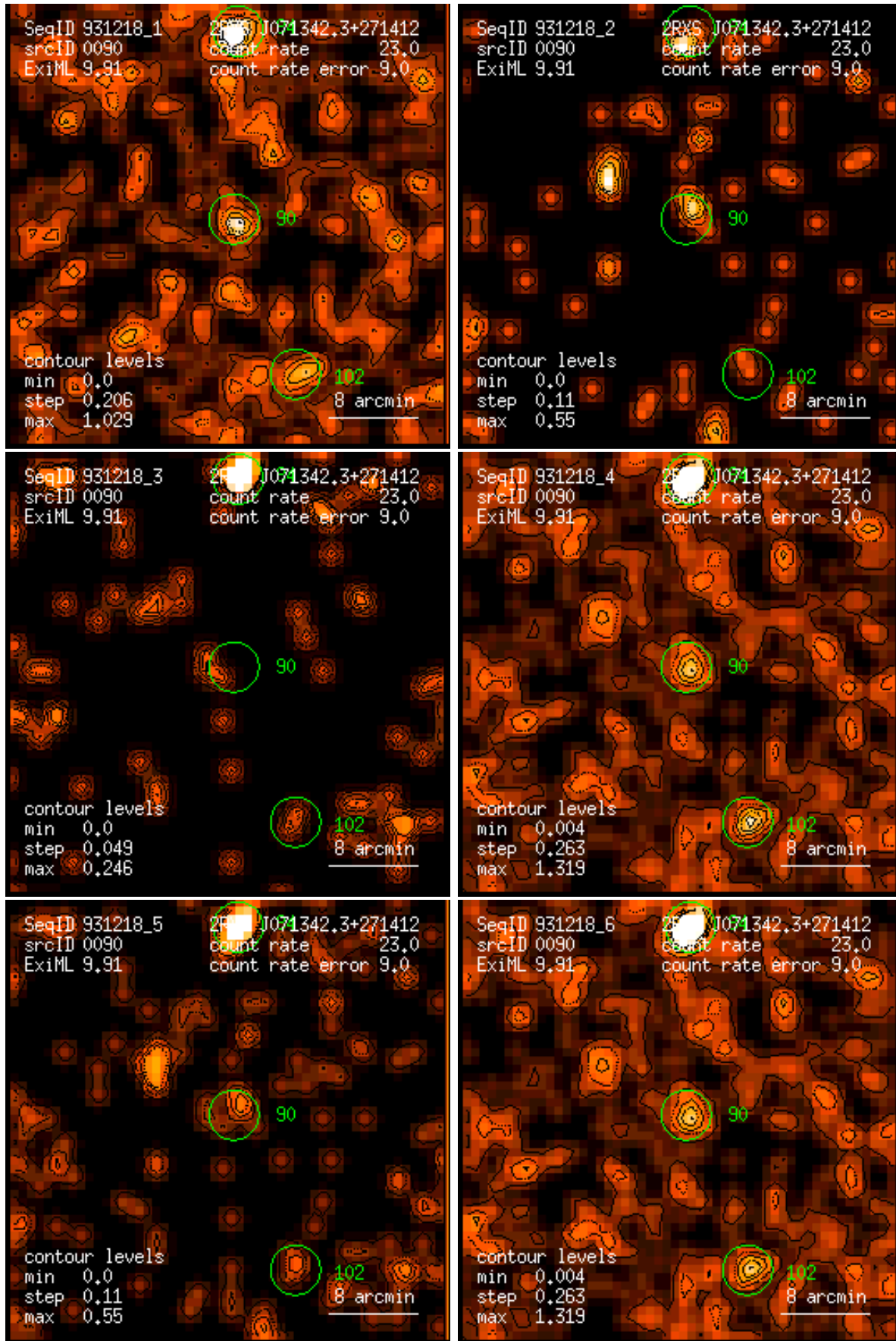
Figure 90: RASS 931218: detection 0090: band rate images, Gaussian filter: (1) PSPC channels 11 – 41, (2) 52 – 90, (3) 91 – 201, (4) 11 – 235, (5) 52 – 201, (6) 11 – 201. Broad band rates in counts/ks. Band rate contour levels in counts/ks/arcmin 2 .
