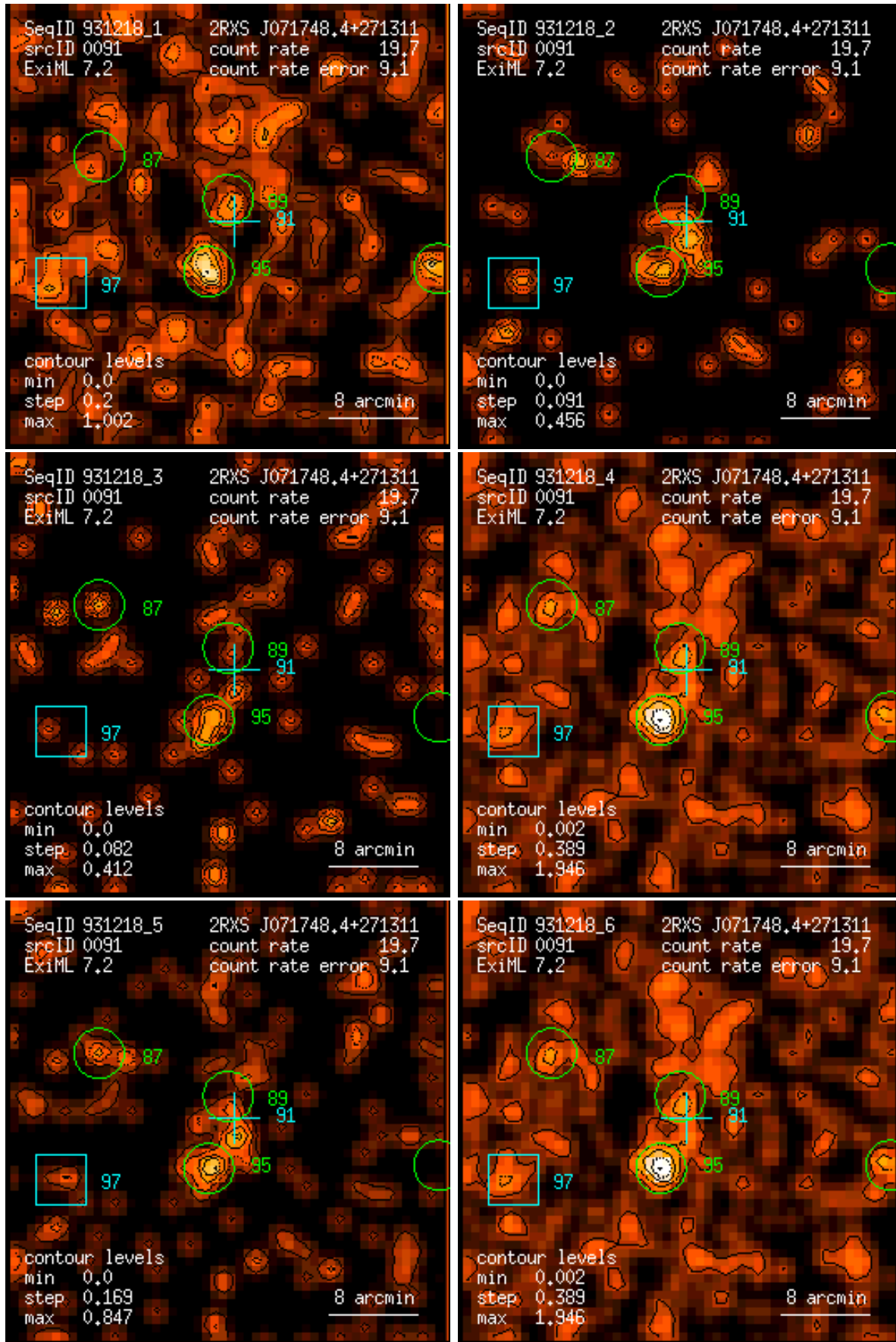
Figure 91: RASS 931218: detection 0091: band rate images, Gaussian filter: (1) PSPC channels 11 – 41, (2) 52 – 90, (3) 91 – 201, (4) 11 – 235, (5) 52 – 201, (6) 11 – 201. Broad band rates in counts/ks. Band rate contour levels in counts/ks/arcmin 2 .
