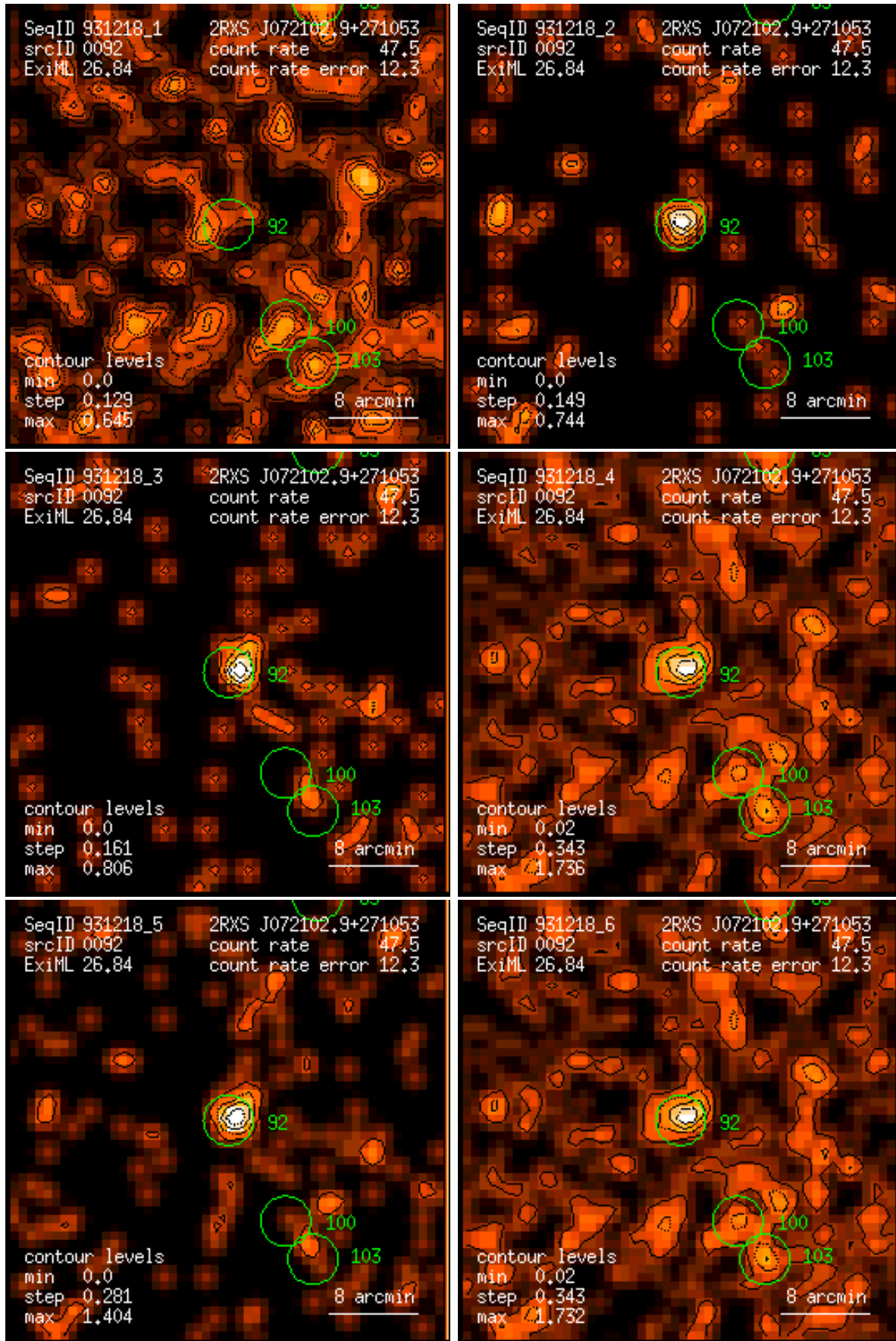
Figure 92: RASS 931218: detection 0092: band rate images, Gaussian filter: (1) PSPC channels 11 – 41, (2) 52 – 90, (3) 91 – 201, (4) 11 – 235, (5) 52 – 201, (6) 11 – 201. Broad band rates in counts/ks. Band rate contour levels in counts/ks/arcmin 2 .
