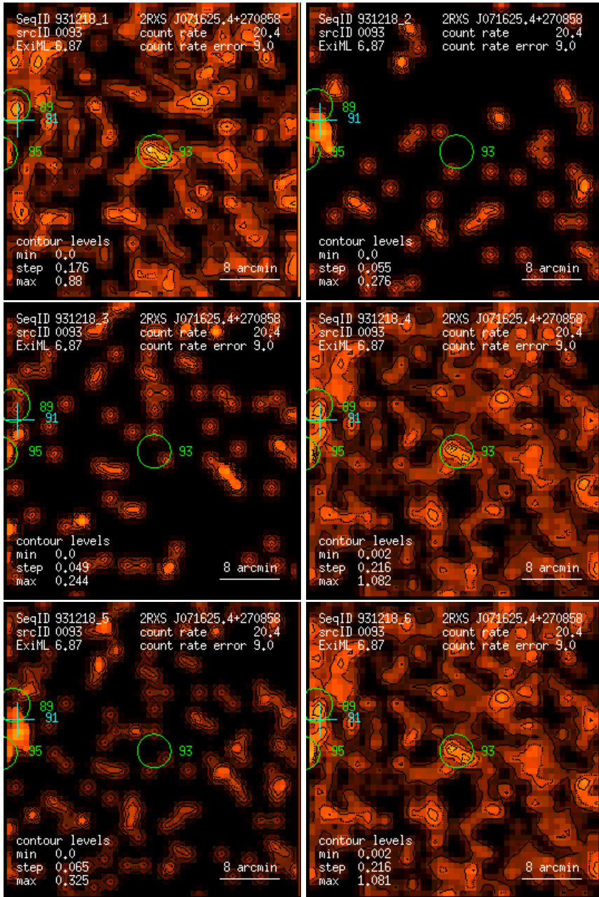
Figure 93: RASS 931218: detection 0093: band rate images, Gaussian filter: (1) PSPC channels 11 – 41, (2) 52 – 90, (3) 91 – 201, (4) 11 – 235, (5) 52 – 201, (6) 11 – 201. Broad band rates in counts/ks. Band rate contour levels in counts/ks/arcmin 2 .
