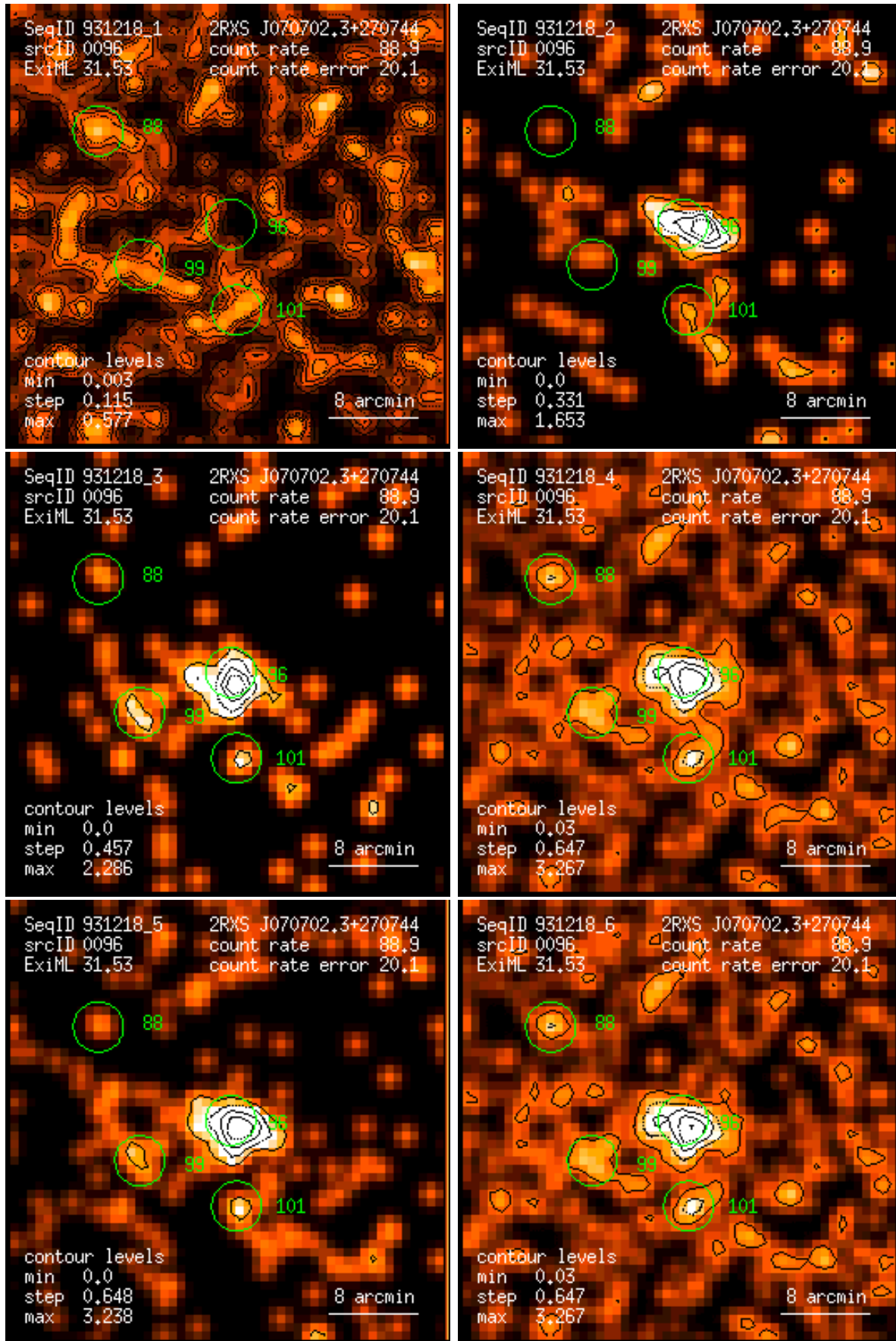
Figure 96: RASS 931218: detection 0096: band rate images, Gaussian filter: (1) PSPC channels 11 – 41, (2) 52 – 90, (3) 91 – 201, (4) 11 – 235, (5) 52 – 201, (6) 11 – 201. Broad band rates in counts/ks. Band rate contour levels in counts/ks/arcmin 2 .
