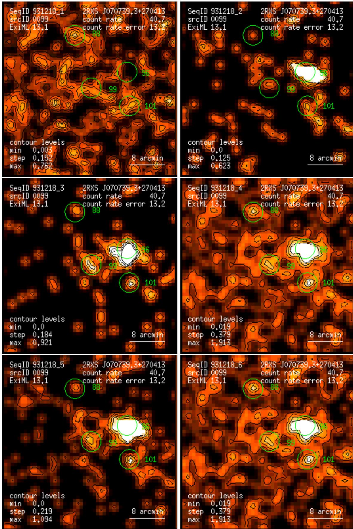
Figure 99: RASS 931218: detection 0099: band rate images, Gaussian filter: (1) PSPC channels 11 – 41, (2) 52 – 90, (3) 91 – 201, (4) 11 – 235, (5) 52 – 201, (6) 11 – 201. Broad band rates in counts/ks. Band rate contour levels in counts/ks/arcmin 2 .
