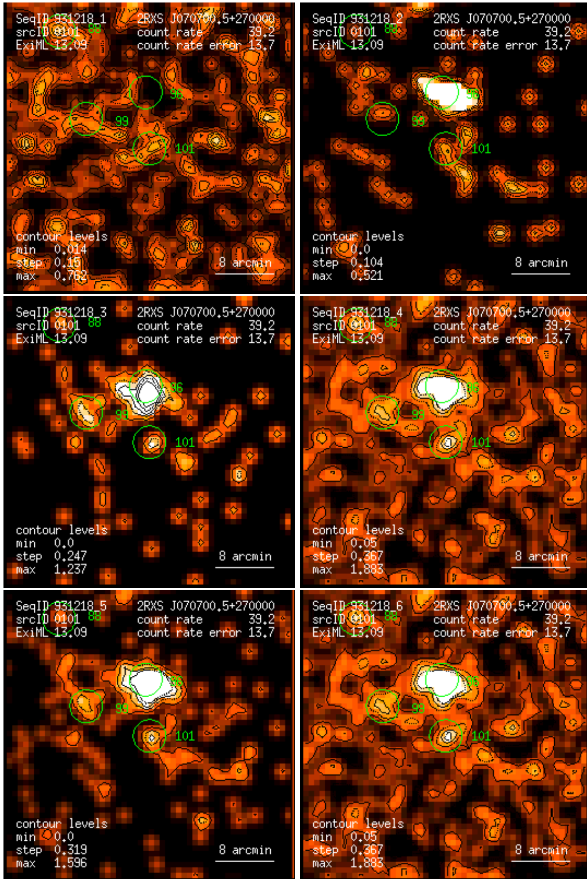
Figure 101: RASS 931218: detection 0101: band rate images, Gaussian filter: (1) PSPC channels 11 – 41, (2) 52 – 90, (3) 91 – 201, (4) 11 – 235, (5) 52 – 201, (6) 11 – 201. Broad band rates in counts/ks. Band rate contour levels in counts/ks/arcmin 2 .
