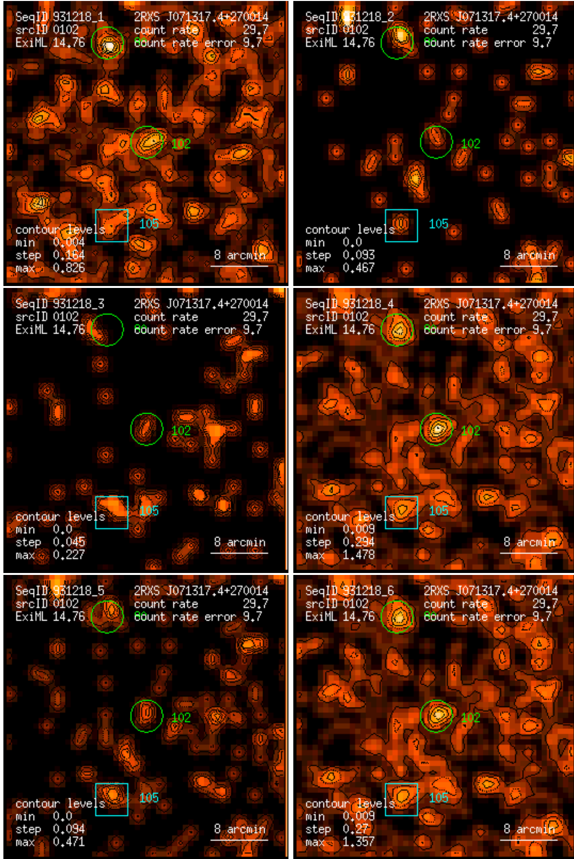
Figure 102: RASS 931218: detection 0102: band rate images, Gaussian filter: (1) PSPC channels 11 – 41, (2) 52 – 90, (3) 91 – 201, (4) 11 – 235, (5) 52 – 201, (6) 11 – 201. Broad band rates in counts/ks. Band rate contour levels in counts/ks/arcmin 2 .
