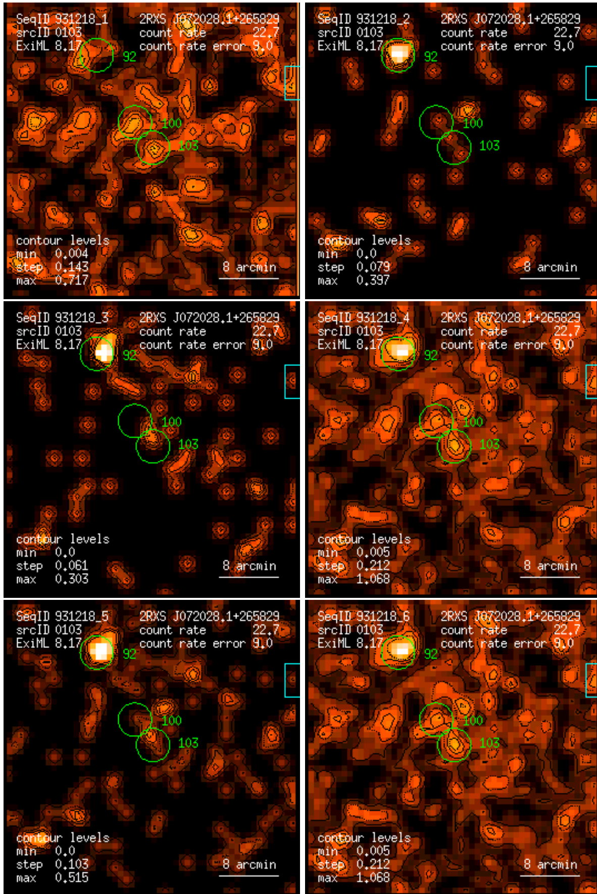
Figure 103: RASS 931218: detection 0103: band rate images, Gaussian filter: (1) PSPC channels 11 – 41, (2) 52 – 90, (3) 91 – 201, (4) 11 – 235, (5) 52 – 201, (6) 11 – 201. Broad band rates in counts/ks. Band rate contour levels in counts/ks/arcmin 2 .
