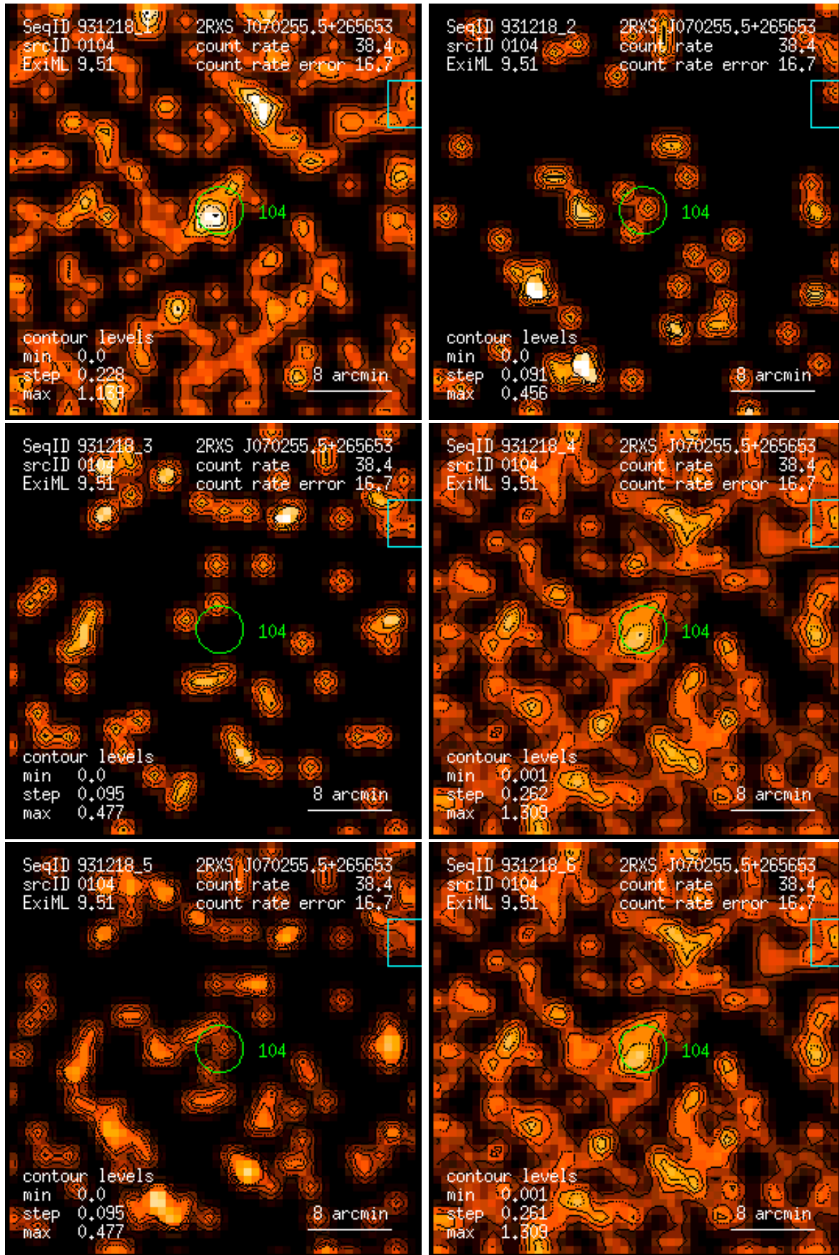
Figure 104: RASS 931218: detection 0104: band rate images, Gaussian filter: (1) PSPC channels 11 – 41, (2) 52 – 90, (3) 91 – 201, (4) 11 – 235, (5) 52 – 201, (6) 11 – 201. Broad band rates in counts/ks. Band rate contour levels in counts/ks/arcmin 2 .
