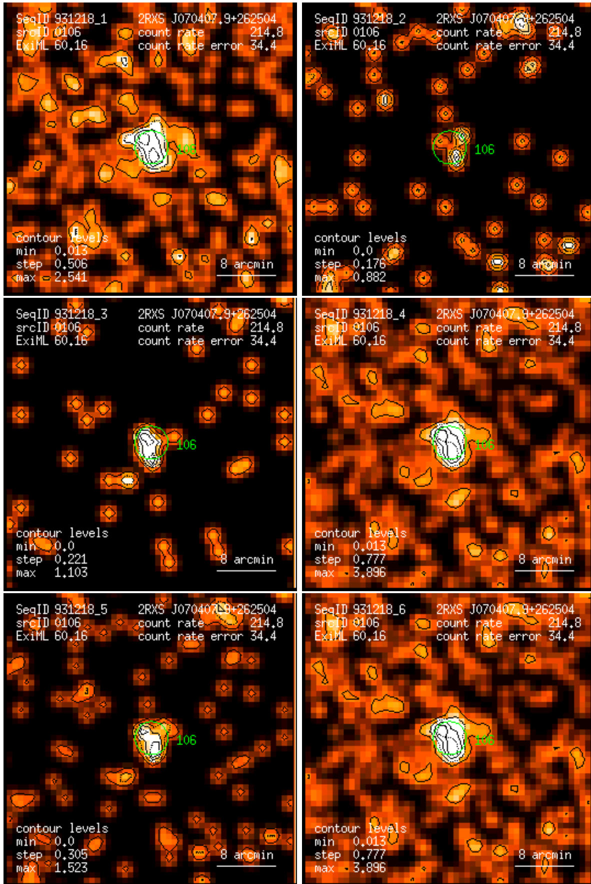
Figure 106: RASS 931218: detection 0106: band rate images, Gaussian filter: (1) PSPC channels 11 – 41, (2) 52 – 90, (3) 91 – 201, (4) 11 – 235, (5) 52 – 201, (6) 11 – 201. Broad band rates in counts/ks. Band rate contour levels in counts/ks/arcmin 2 .
