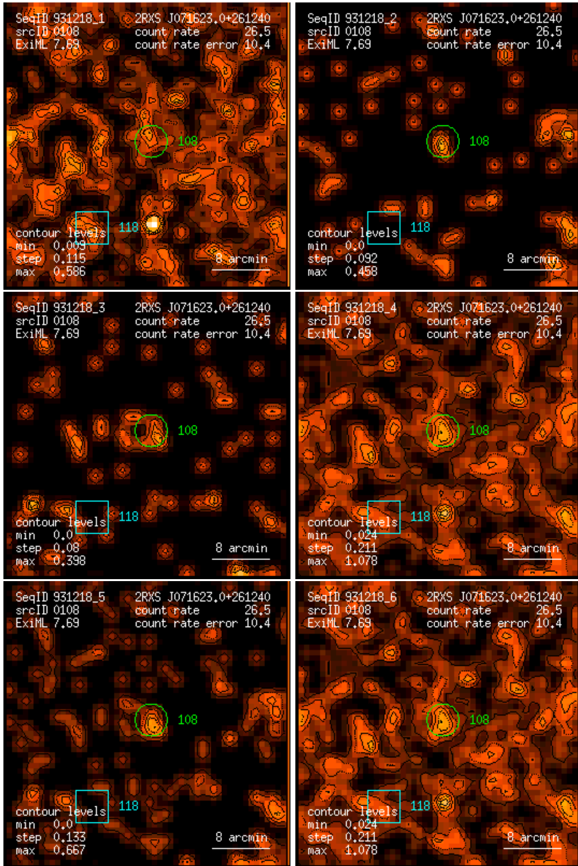
Figure 108: RASS 931218: detection 0108: band rate images, Gaussian filter: (1) PSPC channels 11 – 41, (2) 52 – 90, (3) 91 – 201, (4) 11 – 235, (5) 52 – 201, (6) 11 – 201. Broad band rates in counts/ks. Band rate contour levels in counts/ks/arcmin 2 .
