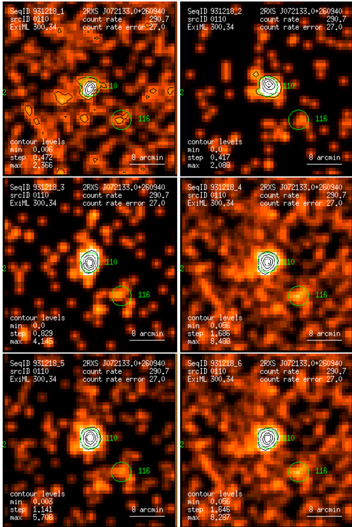
Figure 110: RASS 931218: detection 0110: band rate images, Gaussian filter: (1) PSPC channels 11 – 41, (2) 52 – 90, (3) 91 – 201, (4) 11 – 235, (5) 52 – 201, (6) 11 – 201. Broad band rates in counts/ks. Band rate contour levels in counts/ks/arcmin 2 .
