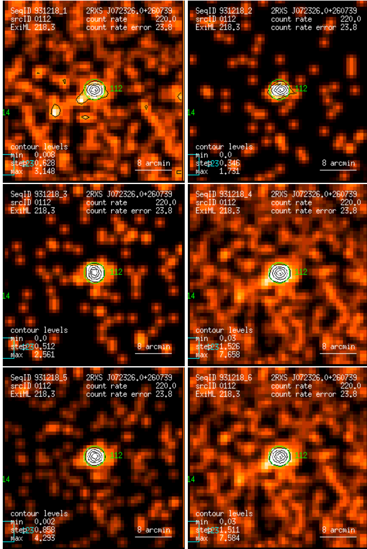
Figure 112: RASS 931218: detection 0112: band rate images, Gaussian filter: (1) PSPC channels 11 – 41, (2) 52 – 90, (3) 91 – 201, (4) 11 – 235, (5) 52 – 201, (6) 11 – 201. Broad band rates in counts/ks. Band rate contour levels in counts/ks/arcmin 2 .
