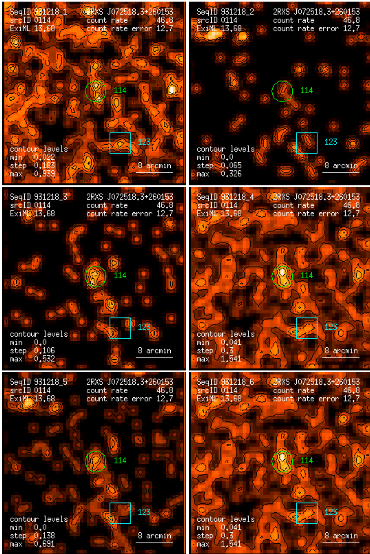
Figure 114: RASS 931218: detection 0114: band rate images, Gaussian filter: (1) PSPC channels 11 – 41, (2) 52 – 90, (3) 91 – 201, (4) 11 – 235, (5) 52 – 201, (6) 11 – 201. Broad band rates in counts/ks. Band rate contour levels in counts/ks/arcmin 2 .
