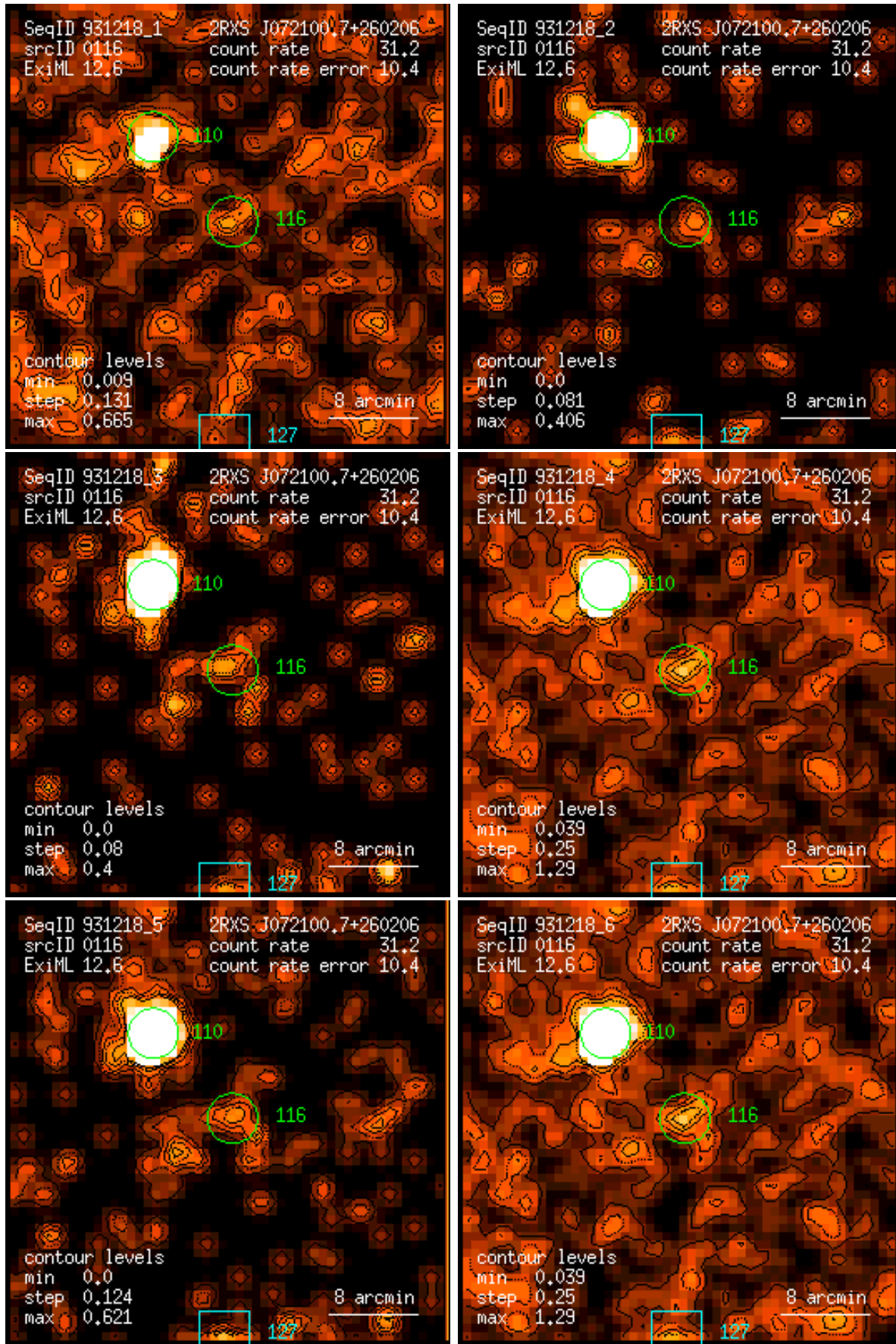
Figure 116: RASS 931218: detection 0116: band rate images, Gaussian filter: (1) PSPC channels 11 – 41, (2) 52 – 90, (3) 91 – 201, (4) 11 – 235, (5) 52 – 201, (6) 11 – 201. Broad band rates in counts/ks. Band rate contour levels in counts/ks/arcmin 2 .
