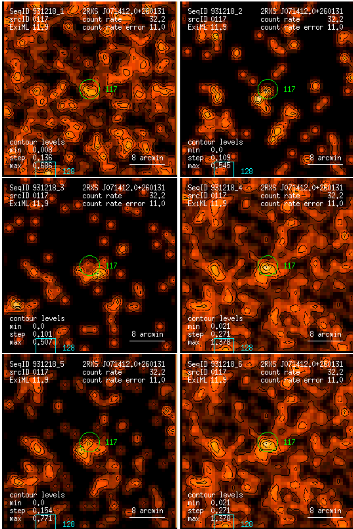
Figure 117: RASS 931218: detection 0117: band rate images, Gaussian filter: (1) PSPC channels 11 – 41, (2) 52 – 90, (3) 91 – 201, (4) 11 – 235, (5) 52 – 201, (6) 11 – 201. Broad band rates in counts/ks. Band rate contour levels in counts/ks/arcmin 2 .
