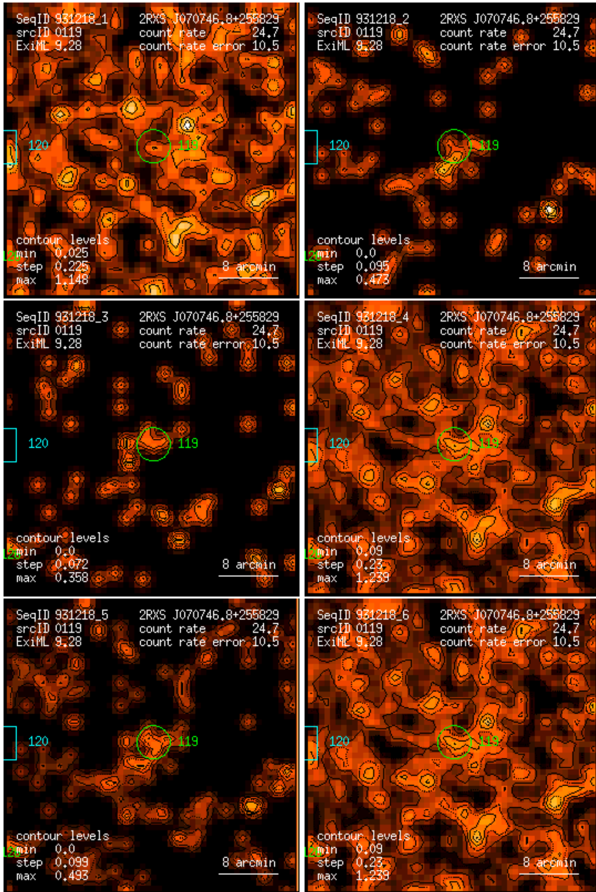
Figure 119: RASS 931218: detection 0119: band rate images, Gaussian filter: (1) PSPC channels 11 – 41, (2) 52 – 90, (3) 91 – 201, (4) 11 – 235, (5) 52 – 201, (6) 11 – 201. Broad band rates in counts/ks. Band rate contour levels in counts/ks/arcmin 2 .
