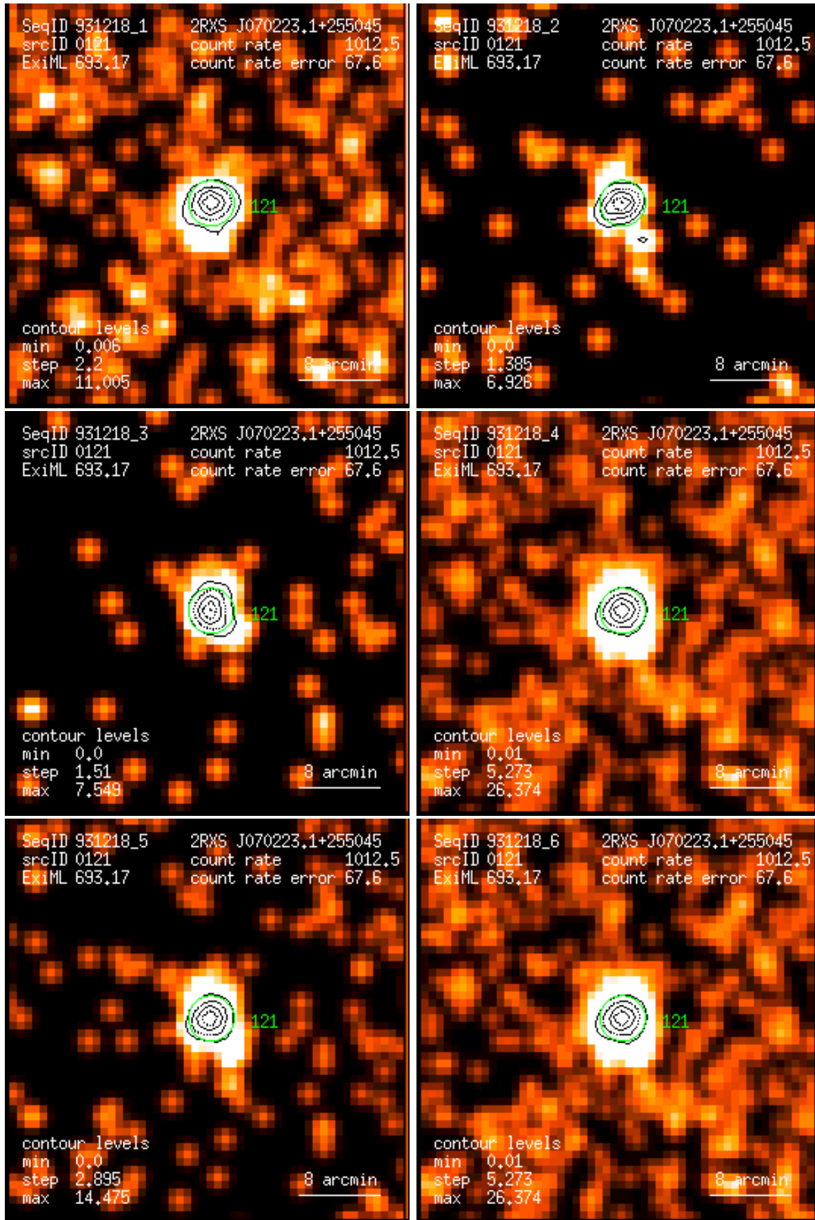
Figure 121: RASS 931218: detection 0121: band rate images, Gaussian filter: (1) PSPC channels 11 – 41, (2) 52 – 90, (3) 91 – 201, (4) 11 – 235, (5) 52 – 201, (6) 11 – 201. Broad band rates in counts/ks. Band rate contour levels in counts/ks/arcmin 2 .
