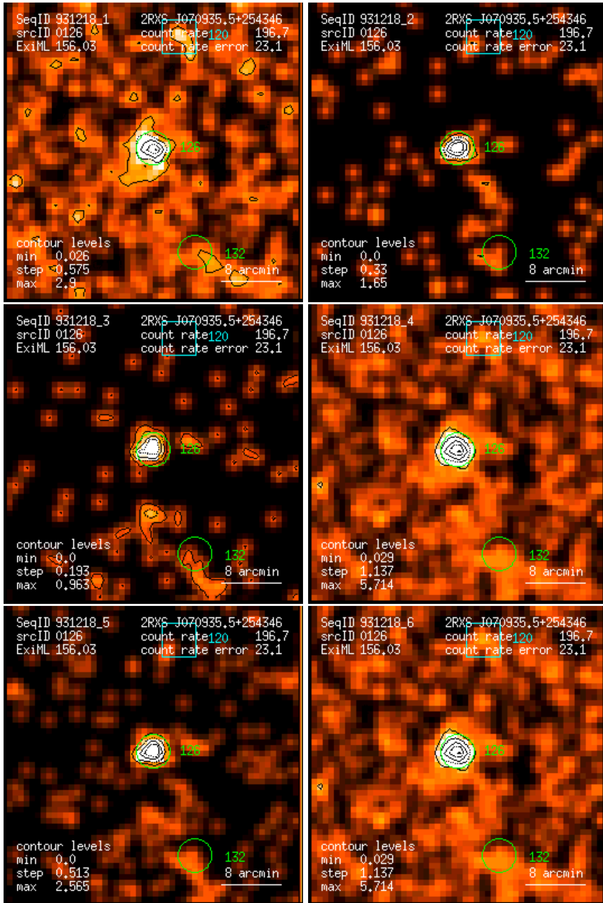
Figure 126: RASS 931218: detection 0126: band rate images, Gaussian filter: (1) PSPC channels 11 – 41, (2) 52 – 90, (3) 91 – 201, (4) 11 – 235, (5) 52 – 201, (6) 11 – 201. Broad band rates in counts/ks. Band rate contour levels in counts/ks/arcmin 2 .
