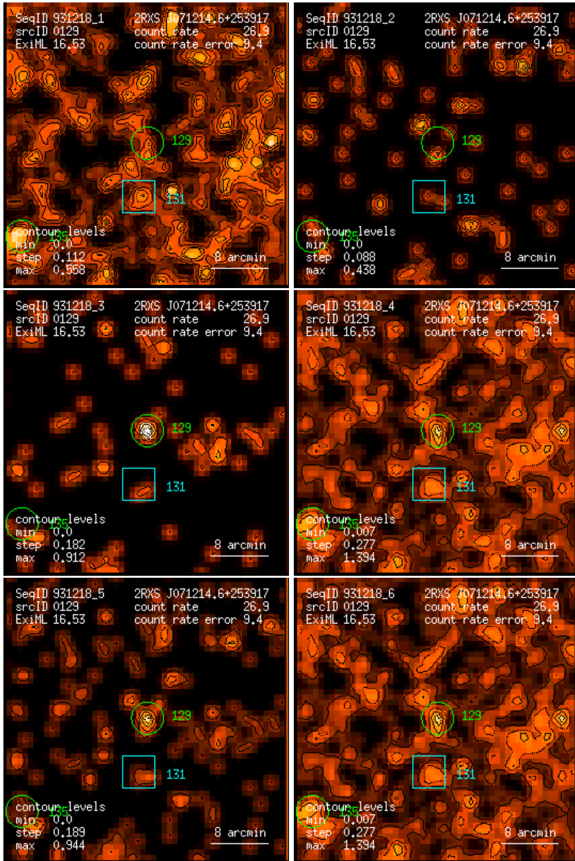
Figure 129: RASS 931218: detection 0129: band rate images, Gaussian filter: (1) PSPC channels 11 – 41, (2) 52 – 90, (3) 91 – 201, (4) 11 – 235, (5) 52 – 201, (6) 11 – 201. Broad band rates in counts/ks. Band rate contour levels in counts/ks/arcmin 2 .
