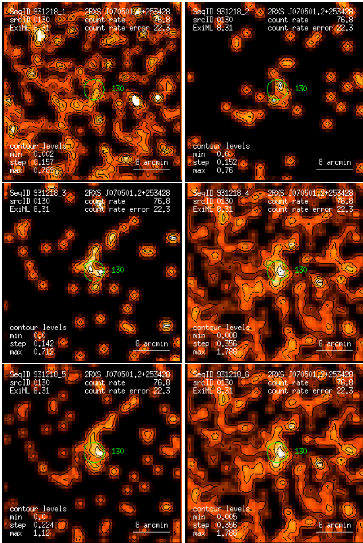
Figure 130: RASS 931218: detection 0130: band rate images, Gaussian filter: (1) PSPC channels 11 – 41, (2) 52 – 90, (3) 91 – 201, (4) 11 – 235, (5) 52 – 201, (6) 11 – 201. Broad band rates in counts/ks. Band rate contour levels in counts/ks/arcmin 2 .
