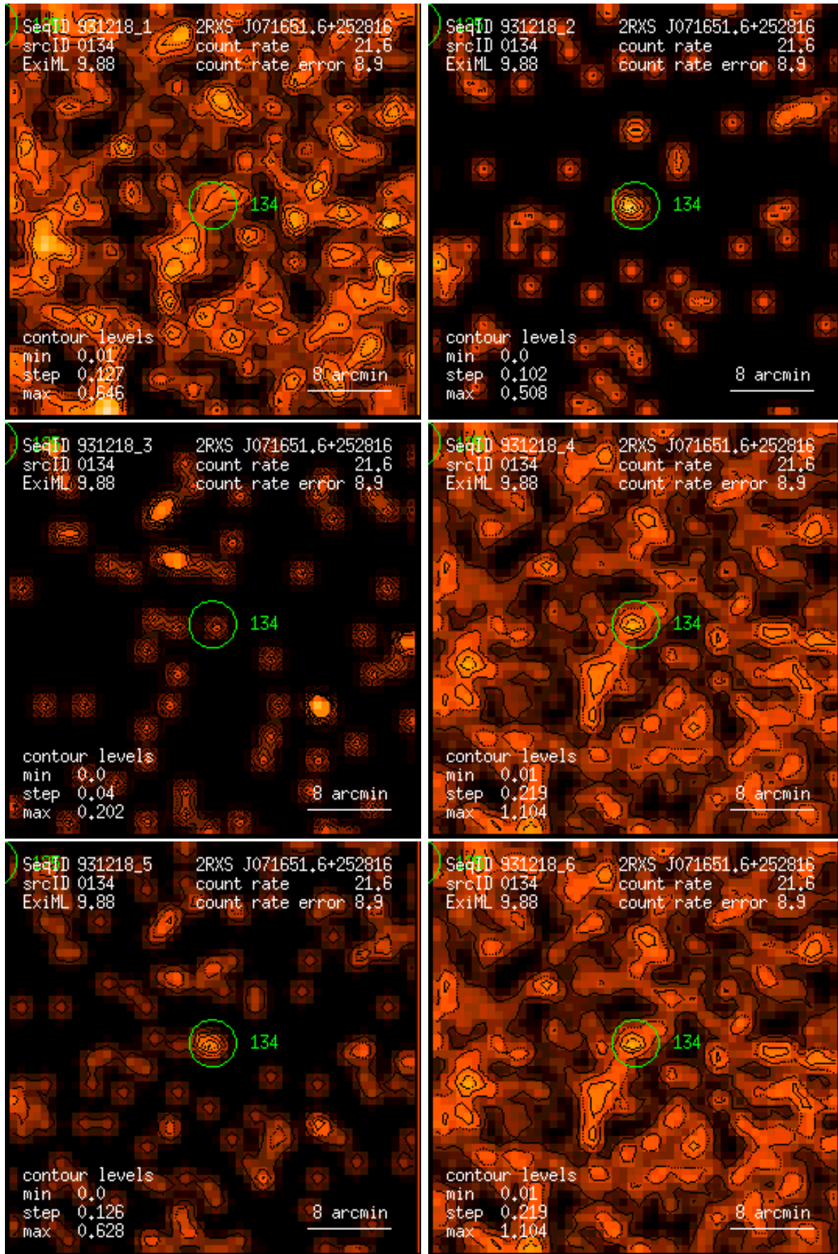
Figure 134: RASS 931218: detection 0134: band rate images, Gaussian filter: (1) PSPC channels 11 – 41, (2) 52 – 90, (3) 91 – 201, (4) 11 – 235, (5) 52 – 201, (6) 11 – 201. Broad band rates in counts/ks. Band rate contour levels in counts/ks/arcmin 2 .
