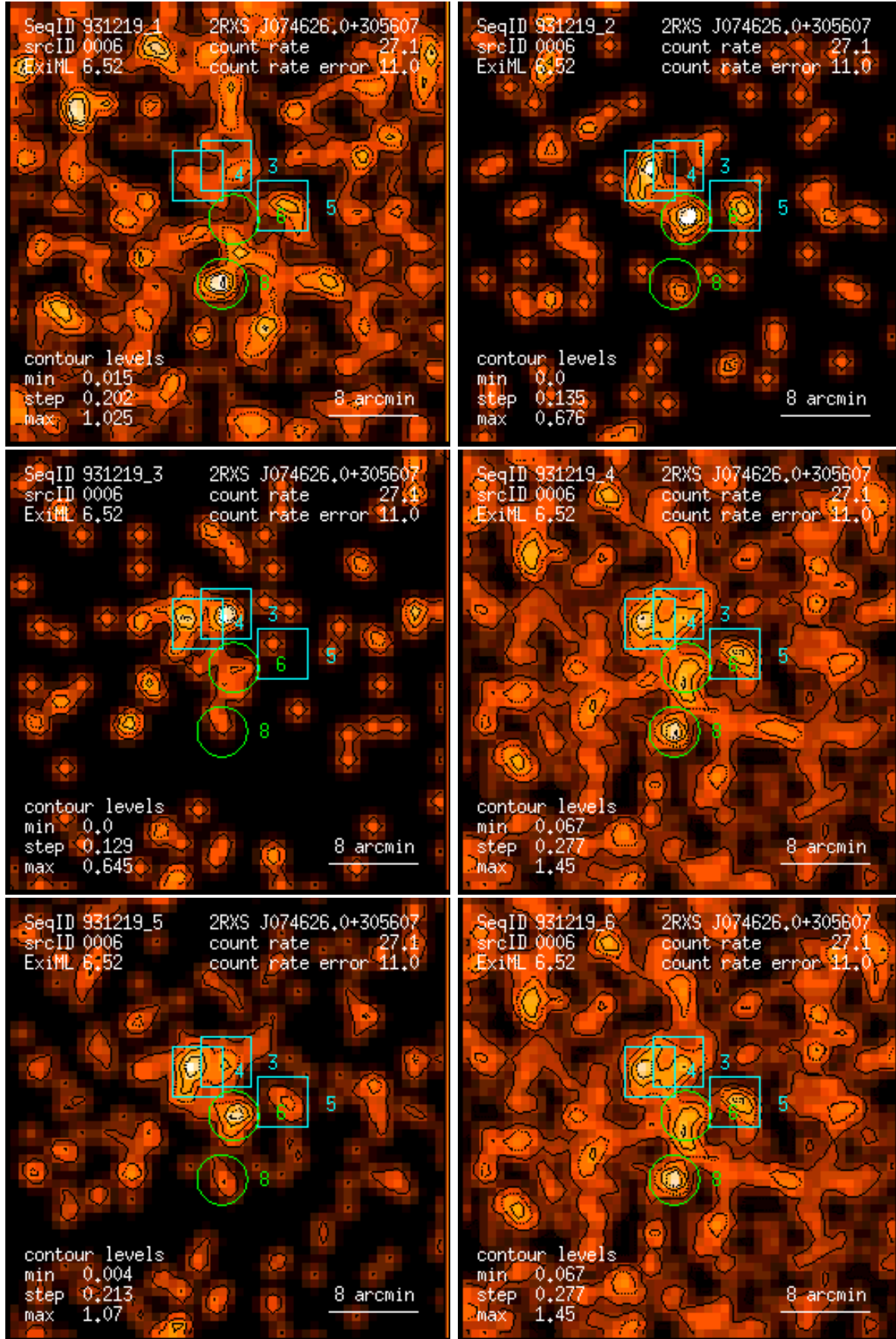
Figure 6: RASS 931219: detection 0006: band rate images, Gaussian filter: (1) PSPC channels 11 – 41, (2) 52 – 90, (3) 91 – 201, (4) 11 – 235, (5) 52 – 201, (6) 11 – 201. Broad band rates in counts/ks. Band rate contour levels in counts/ks/arcmin 2 .
