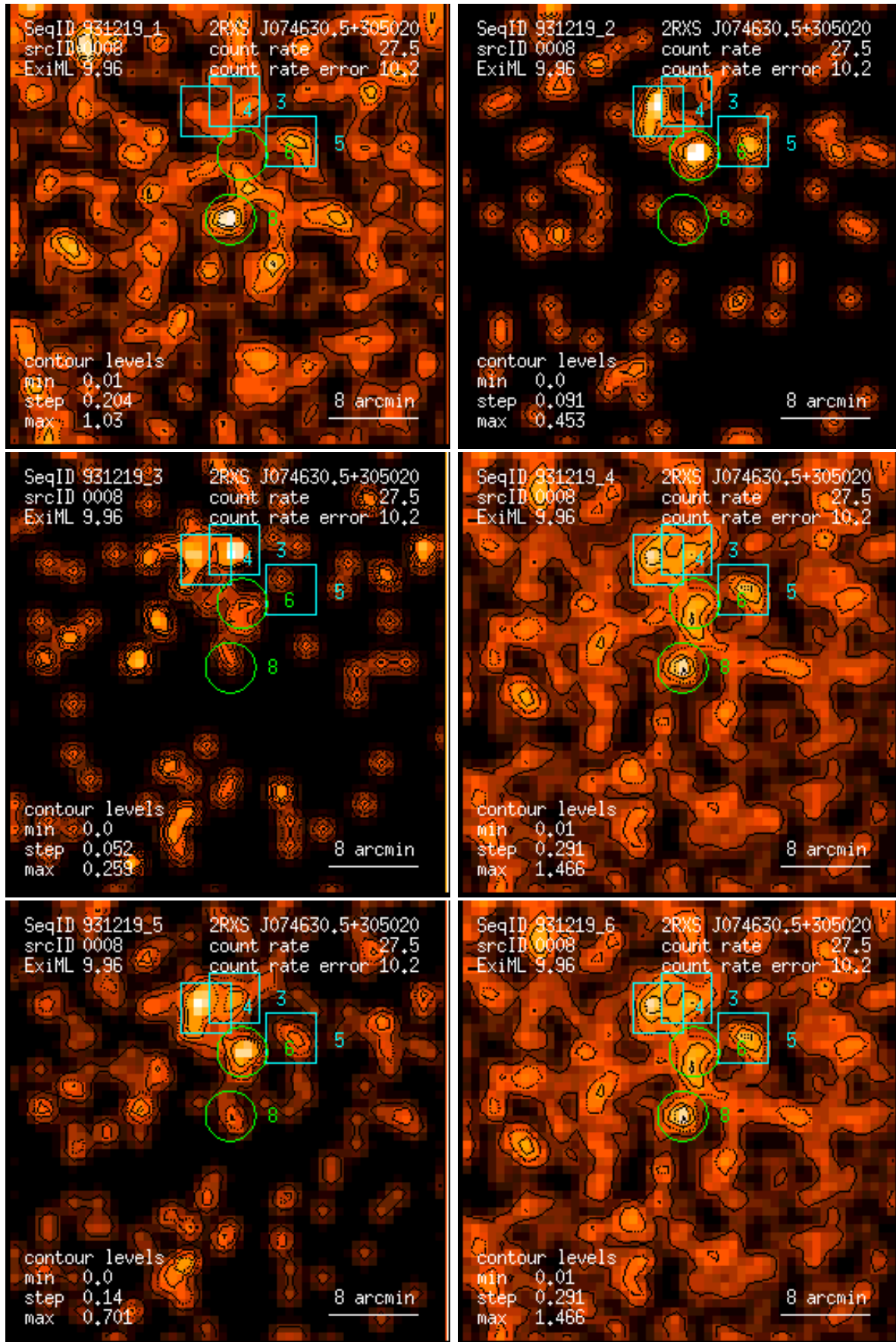
Figure 8: RASS 931219: detection 0008: band rate images, Gaussian filter: (1) PSPC channels 11 – 41, (2) 52 – 90, (3) 91 – 201, (4) 11 – 235, (5) 52 – 201, (6) 11 – 201. Broad band rates in counts/ks. Band rate contour levels in counts/ks/arcmin 2 .
