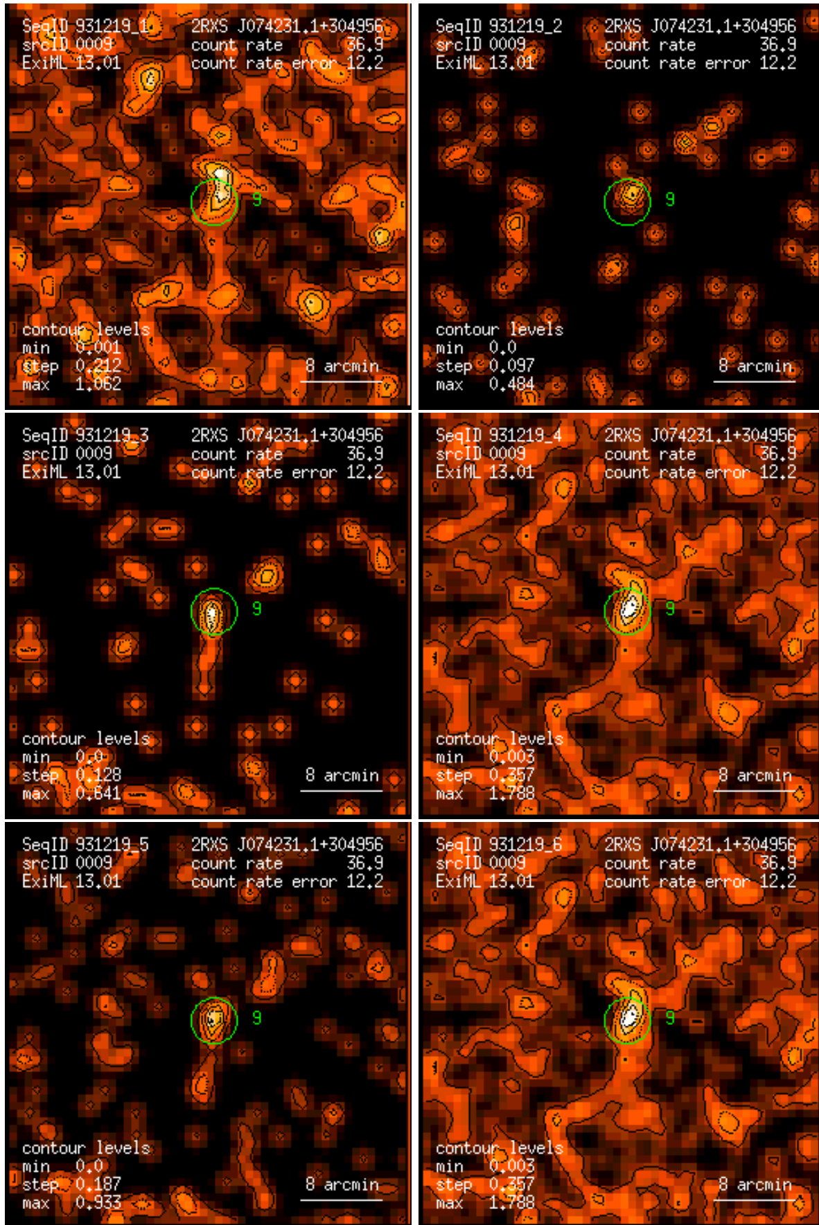
Figure 9: RASS 931219: detection 0009: band rate images, Gaussian filter: (1) PSPC channels 11 – 41, (2) 52 – 90, (3) 91 – 201, (4) 11 – 235, (5) 52 – 201, (6) 11 – 201. Broad band rates in counts/ks. Band rate contour levels in counts/ks/arcmin 2 .
