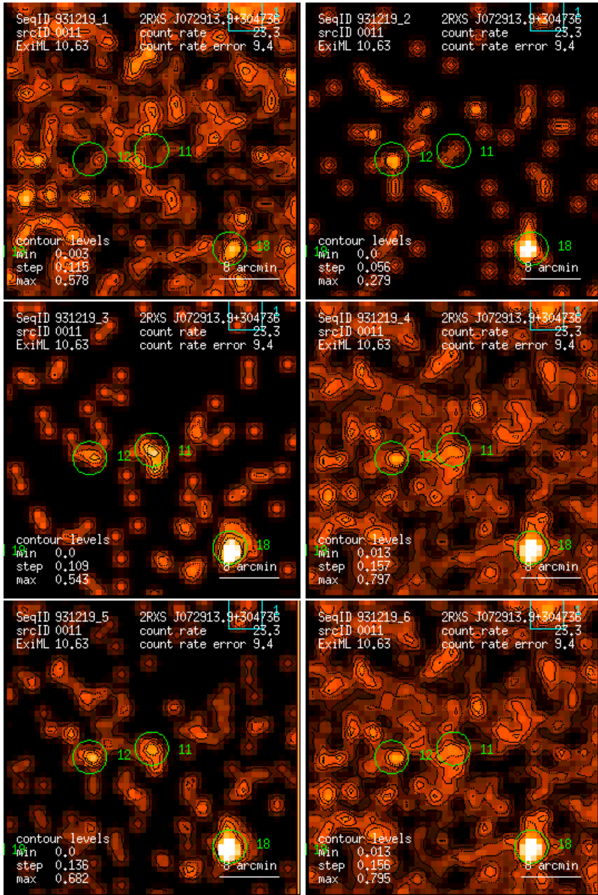
Figure 11: RASS 931219: detection 0011: band rate images, Gaussian filter: (1) PSPC channels 11 – 41, (2) 52 – 90, (3) 91 – 201, (4) 11 – 235, (5) 52 – 201, (6) 11 – 201. Broad band rates in counts/ks. Band rate contour levels in counts/ks/arcmin 2 .
