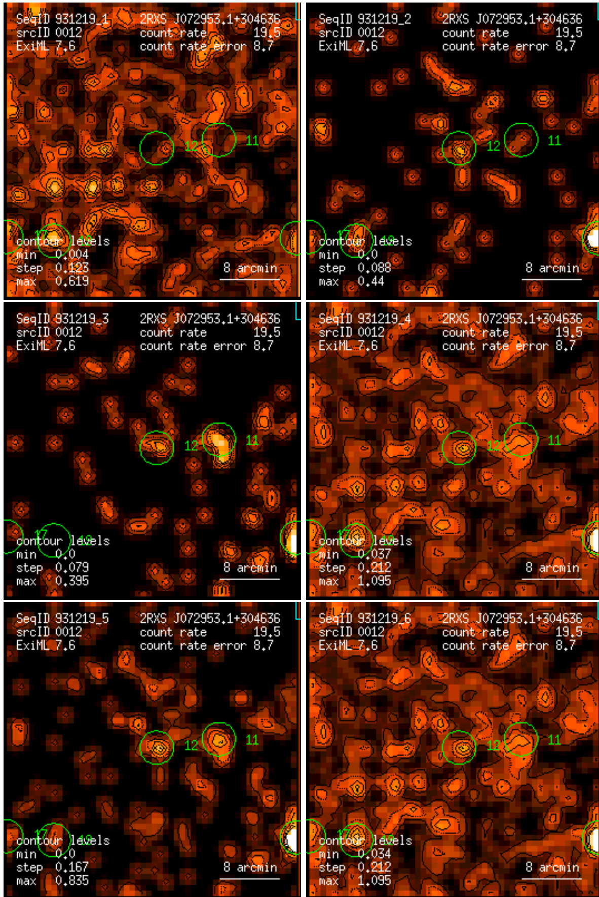
Figure 12: RASS 931219: detection 0012: band rate images, Gaussian filter: (1) PSPC channels 11 – 41, (2) 52 – 90, (3) 91 – 201, (4) 11 – 235, (5) 52 – 201, (6) 11 – 201. Broad band rates in counts/ks. Band rate contour levels in counts/ks/arcmin 2 .
