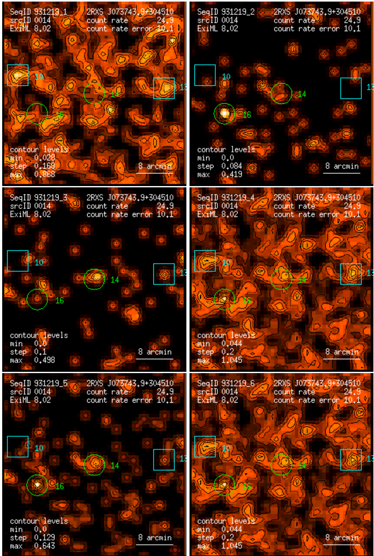
Figure 14: RASS 931219: detection 0014: band rate images, Gaussian filter: (1) PSPC channels 11 – 41, (2) 52 – 90, (3) 91 – 201, (4) 11 – 235, (5) 52 – 201, (6) 11 – 201. Broad band rates in counts/ks. Band rate contour levels in counts/ks/arcmin 2 .
