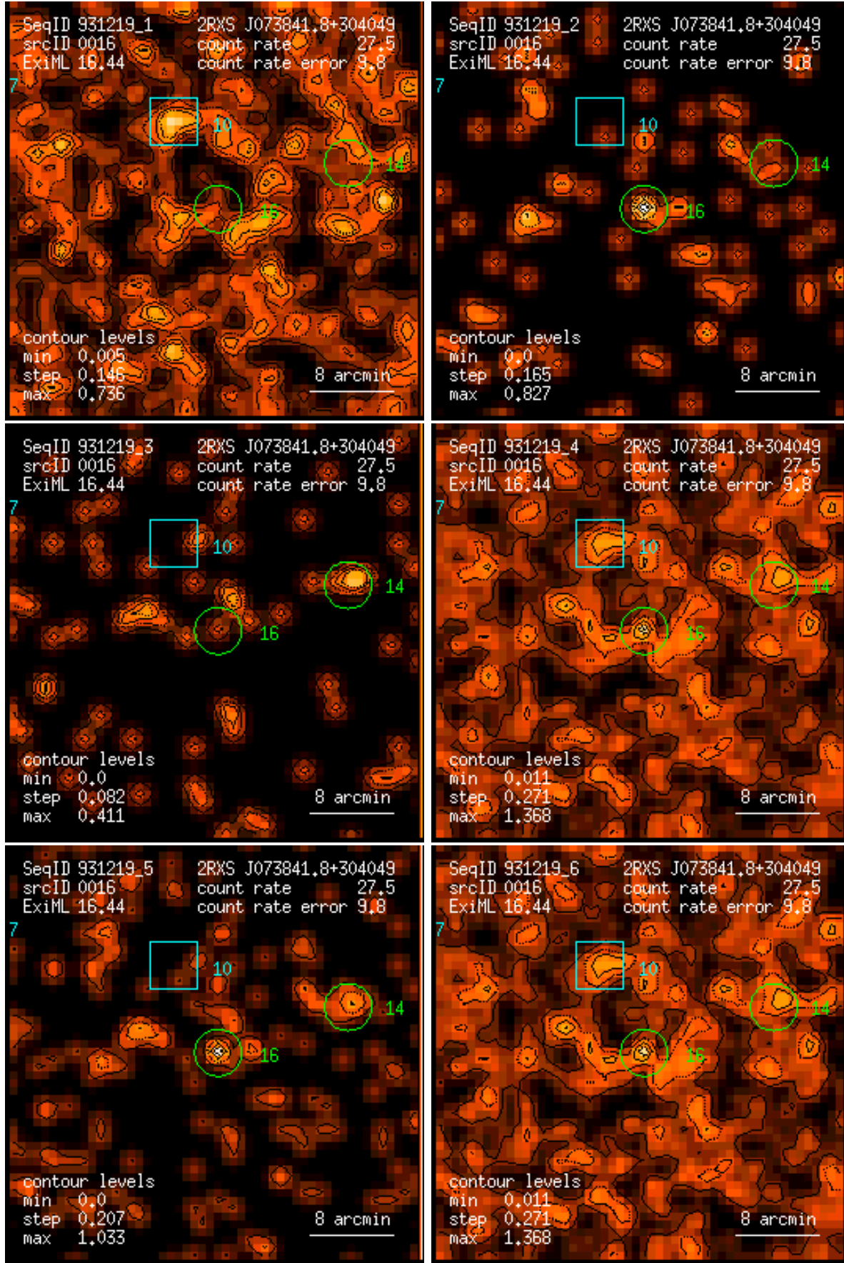
Figure 16: RASS 931219: detection 0016: band rate images, Gaussian filter: (1) PSPC channels 11 – 41, (2) 52 – 90, (3) 91 – 201, (4) 11 – 235, (5) 52 – 201, (6) 11 – 201. Broad band rates in counts/ks. Band rate contour levels in counts/ks/arcmin 2 .
