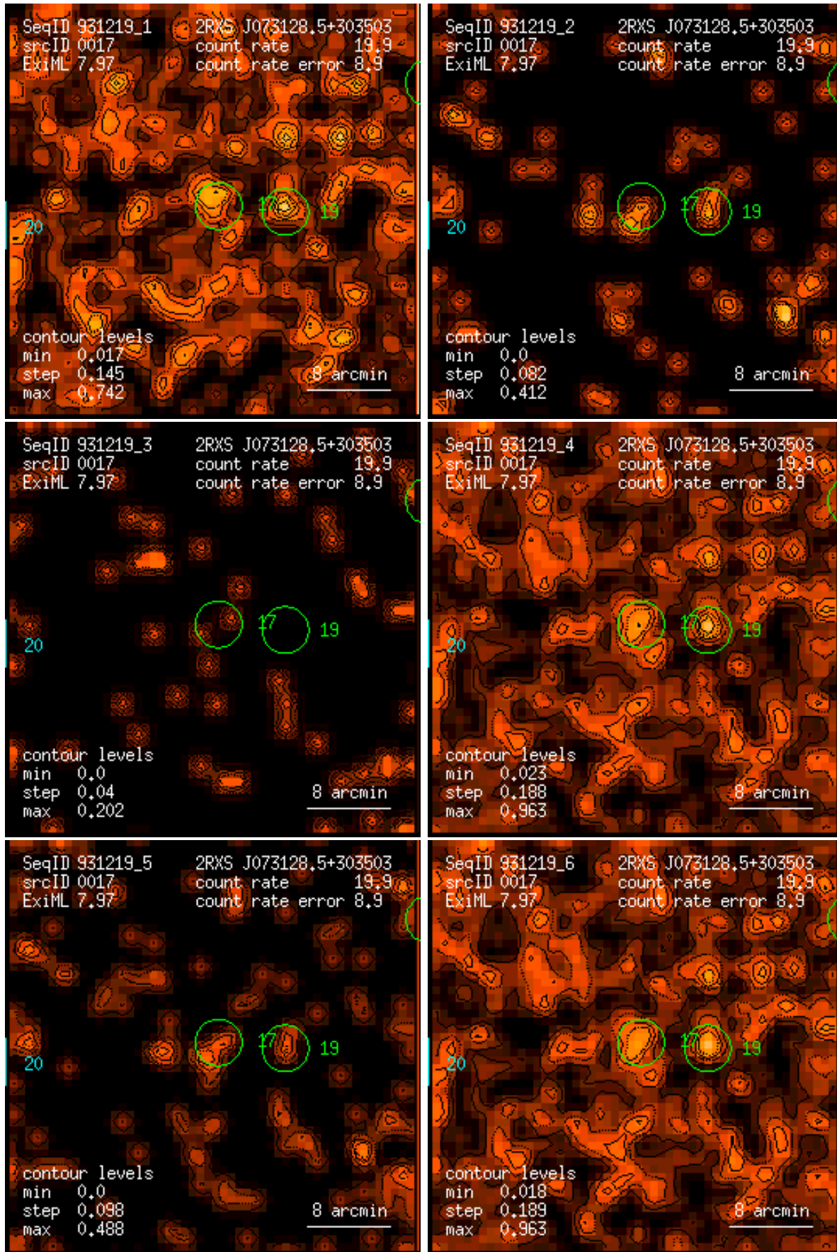
Figure 17: RASS 931219: detection 0017: band rate images, Gaussian filter: (1) PSPC channels 11 – 41, (2) 52 – 90, (3) 91 – 201, (4) 11 – 235, (5) 52 – 201, (6) 11 – 201. Broad band rates in counts/ks. Band rate contour levels in counts/ks/arcmin 2 .
