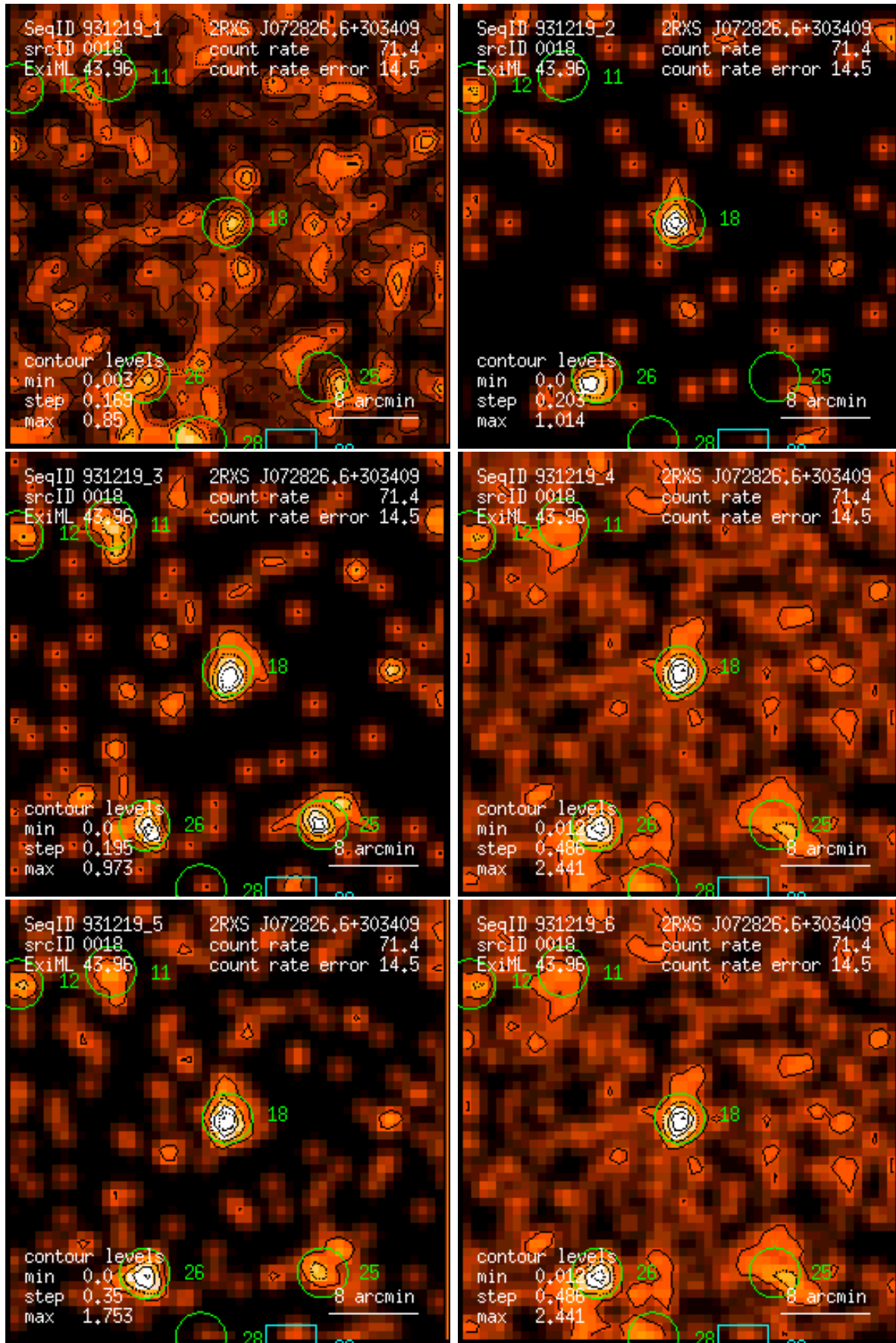
Figure 18: RASS 931219: detection 0018: band rate images, Gaussian filter: (1) PSPC channels 11 – 41, (2) 52 – 90, (3) 91 – 201, (4) 11 – 235, (5) 52 – 201, (6) 11 – 201. Broad band rates in counts/ks. Band rate contour levels in counts/ks/arcmin 2 .
