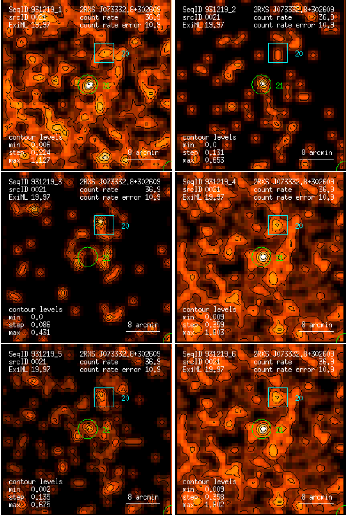
Figure 21: RASS 931219: detection 0021: band rate images, Gaussian filter: (1) PSPC channels 11 – 41, (2) 52 – 90, (3) 91 – 201, (4) 11 – 235, (5) 52 – 201, (6) 11 – 201. Broad band rates in counts/ks. Band rate contour levels in counts/ks/arcmin 2 .
