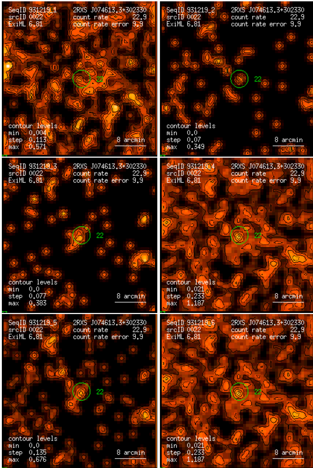
Figure 22: RASS 931219: detection 0022: band rate images, Gaussian filter: (1) PSPC channels 11 – 41, (2) 52 – 90, (3) 91 – 201, (4) 11 – 235, (5) 52 – 201, (6) 11 – 201. Broad band rates in counts/ks. Band rate contour levels in counts/ks/arcmin 2 .
